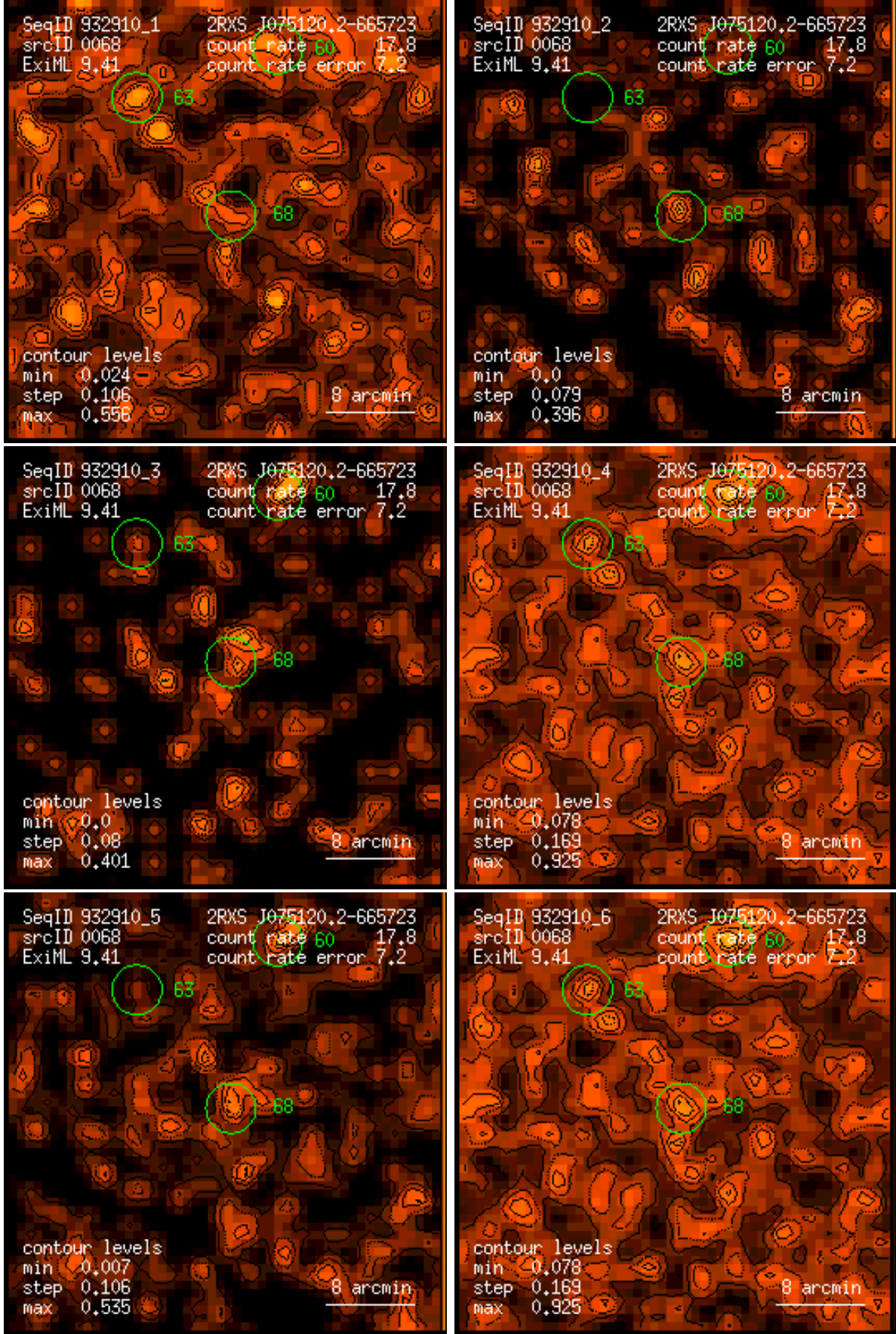
Figure 68: RASS 932910: detection 0068: band rate images, Gaussian filter: (1) PSPC channels 11 – 41, (2) 52 – 90, (3) 91 – 201, (4) 11 – 235, (5) 52 – 201, (6) 11 – 201. Broad band rates in counts/ks. Band rate contour levels in counts/ks/arcmin 2 .
