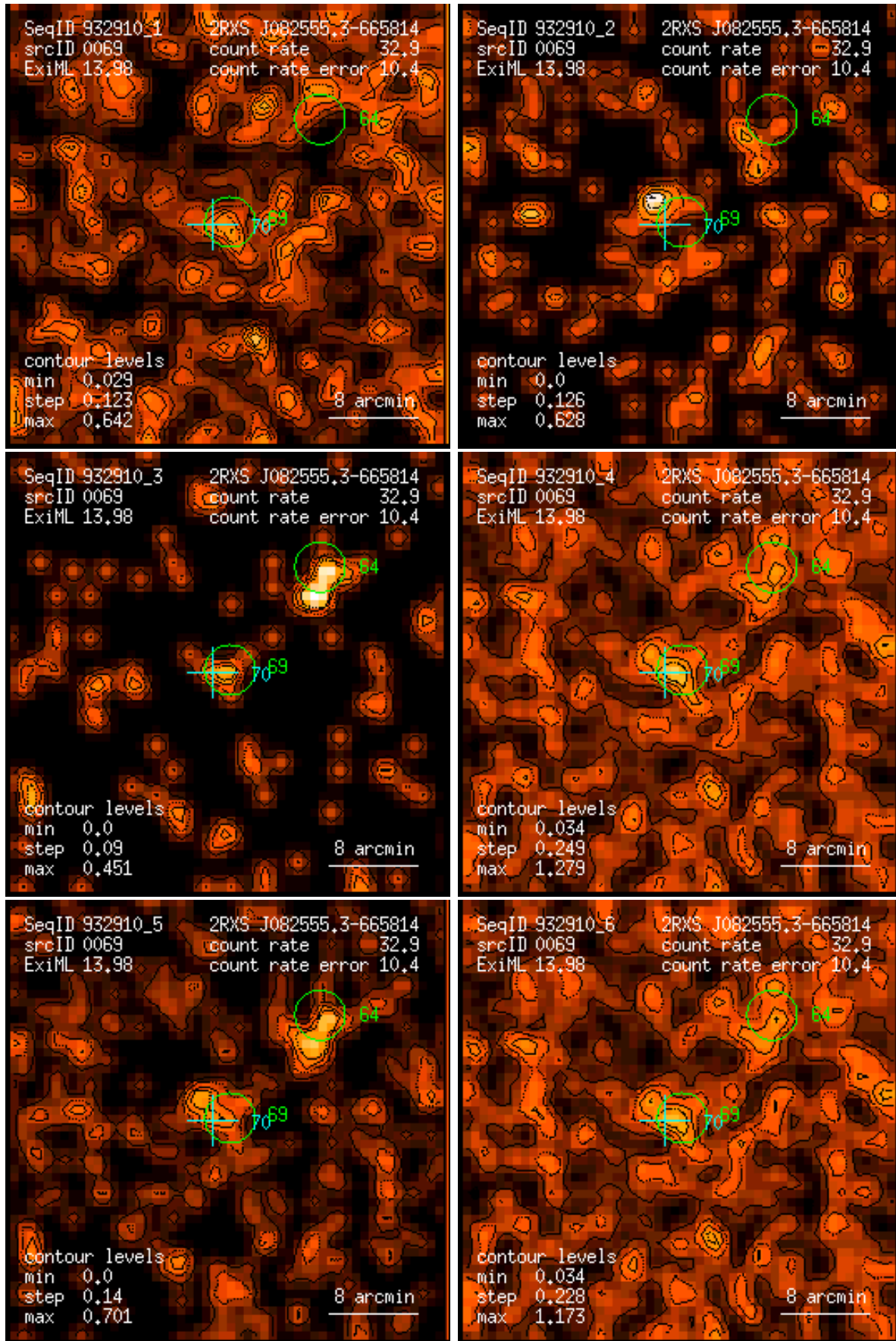
Figure 69: RASS 932910: detection 0069: band rate images, Gaussian filter: (1) PSPC channels 11 – 41, (2) 52 – 90, (3) 91 – 201, (4) 11 – 235, (5) 52 – 201, (6) 11 – 201. Broad band rates in counts/ks. Band rate contour levels in counts/ks/arcmin 2 .
