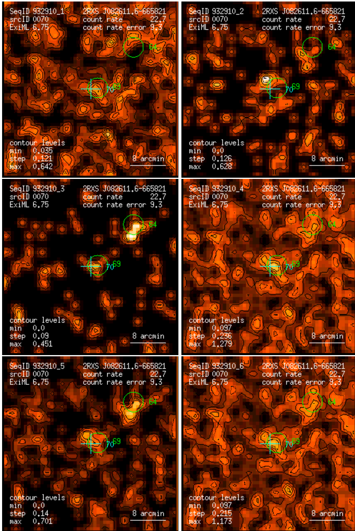
Figure 70: RASS 932910: detection 0070: band rate images, Gaussian filter: (1) PSPC channels 11 – 41, (2) 52 – 90, (3) 91 – 201, (4) 11 – 235, (5) 52 – 201, (6) 11 – 201. Broad band rates in counts/ks. Band rate contour levels in counts/ks/arcmin 2 .
