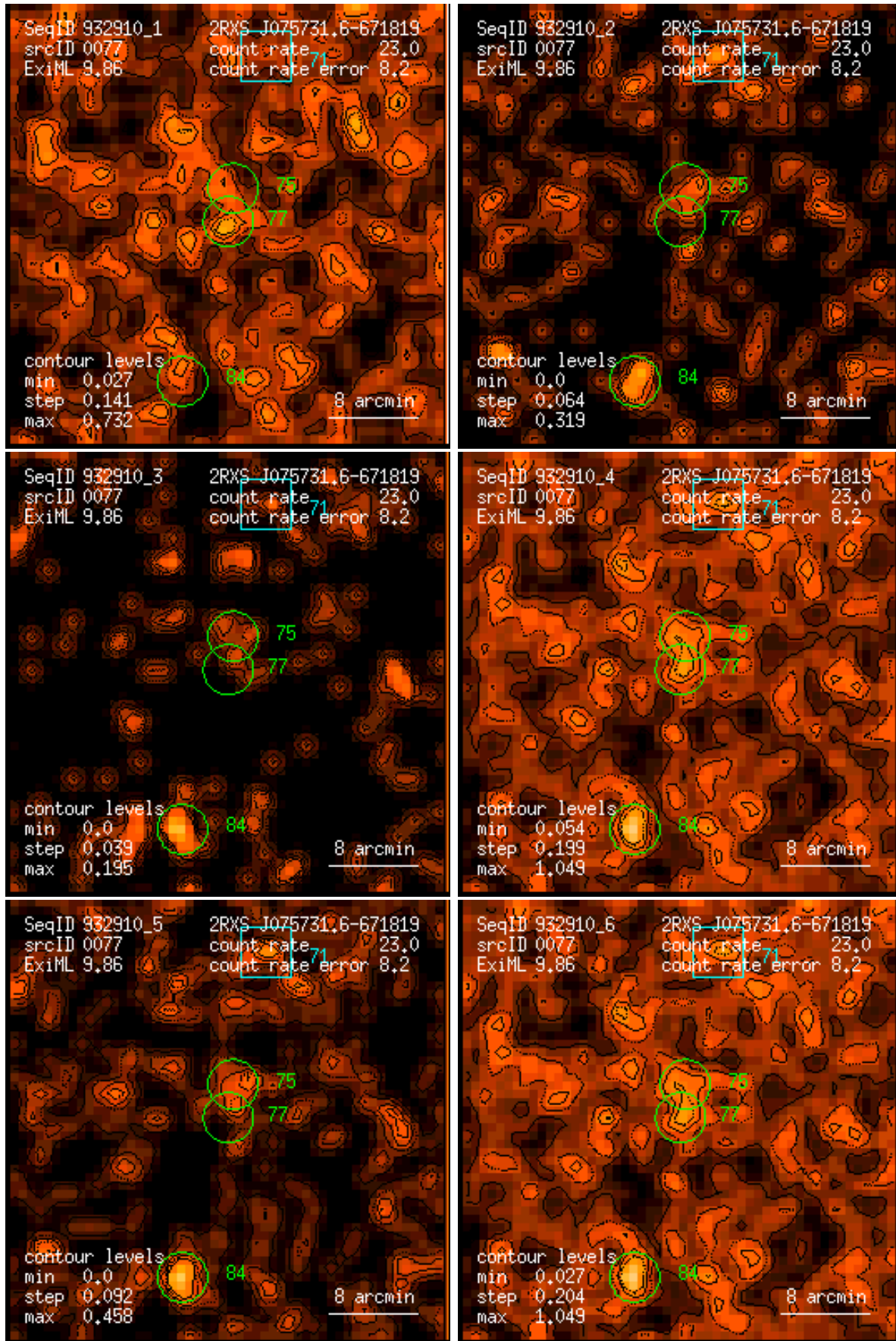
Figure 77: RASS 932910: detection 0077: band rate images, Gaussian filter: (1) PSPC channels 11 – 41, (2) 52 – 90, (3) 91 – 201, (4) 11 – 235, (5) 52 – 201, (6) 11 – 201. Broad band rates in counts/ks. Band rate contour levels in counts/ks/arcmin 2 .
