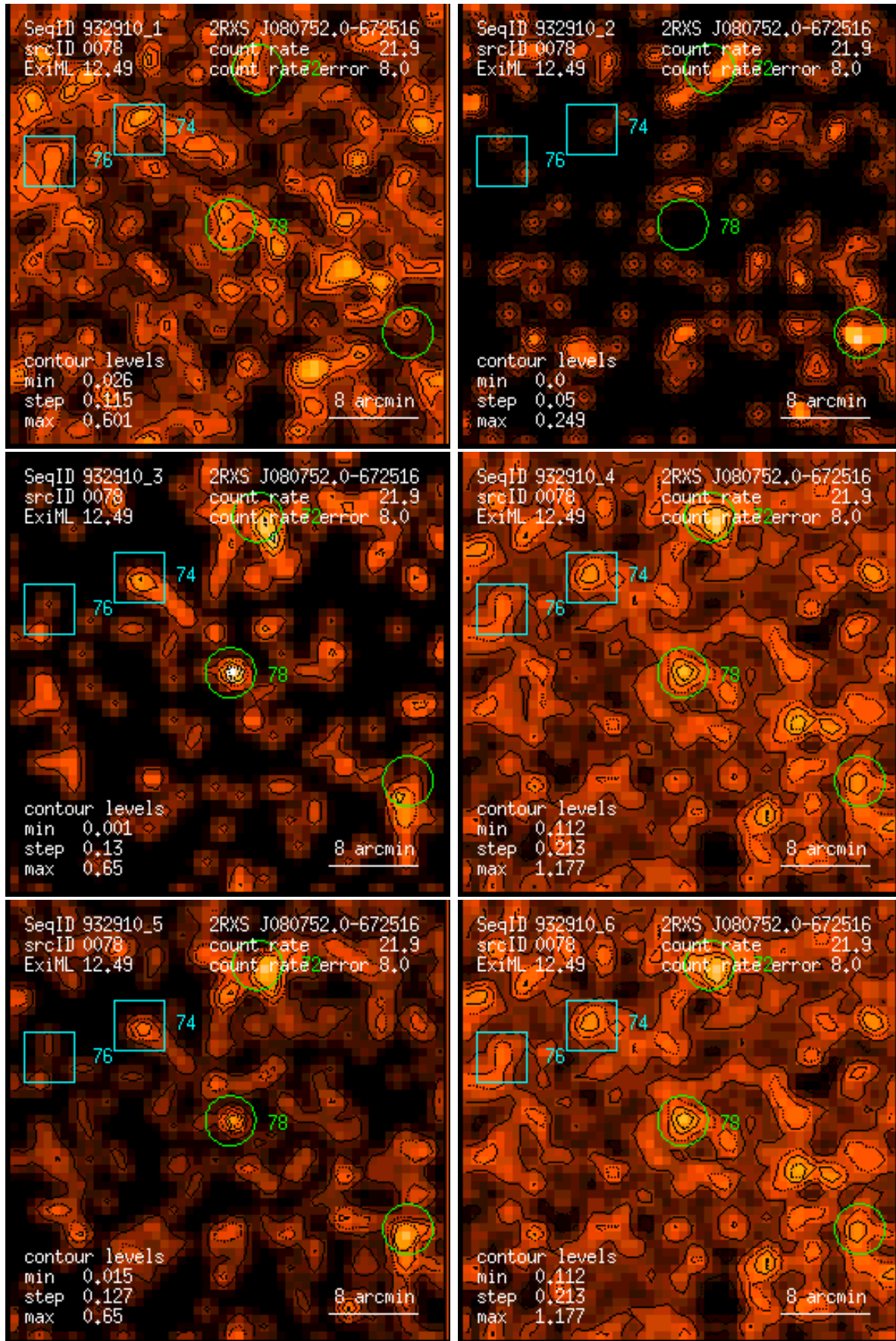
Figure 78: RASS 932910: detection 0078: band rate images, Gaussian filter: (1) PSPC channels 11 – 41, (2) 52 – 90, (3) 91 – 201, (4) 11 – 235, (5) 52 – 201, (6) 11 – 201. Broad band rates in counts/ks. Band rate contour levels in counts/ks/arcmin 2 .
