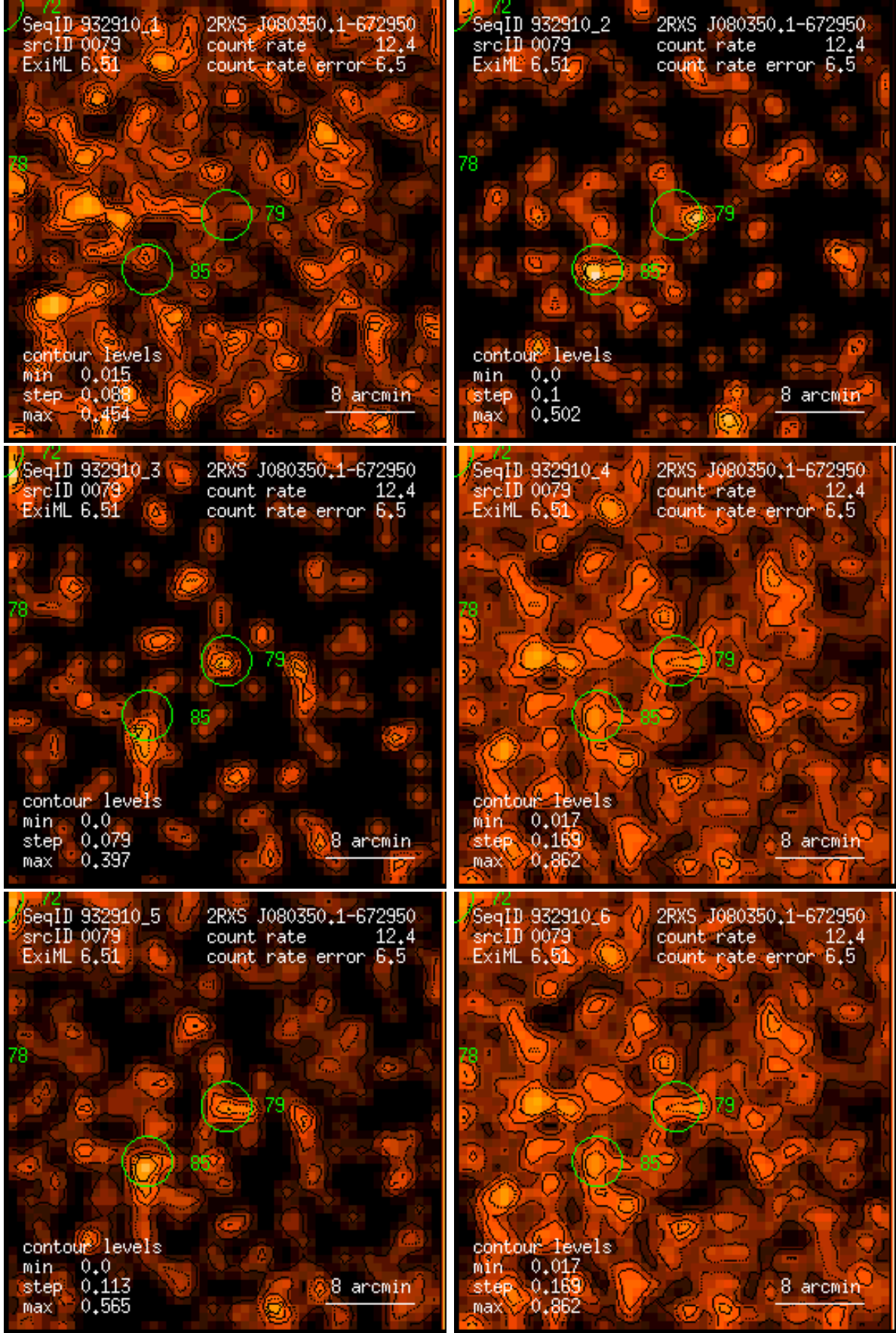
Figure 79: RASS 932910: detection 0079: band rate images, Gaussian filter: (1) PSPC channels 11 – 41, (2) 52 – 90, (3) 91 – 201, (4) 11 – 235, (5) 52 – 201, (6) 11 – 201. Broad band rates in counts/ks. Band rate contour levels in counts/ks/arcmin 2 .
