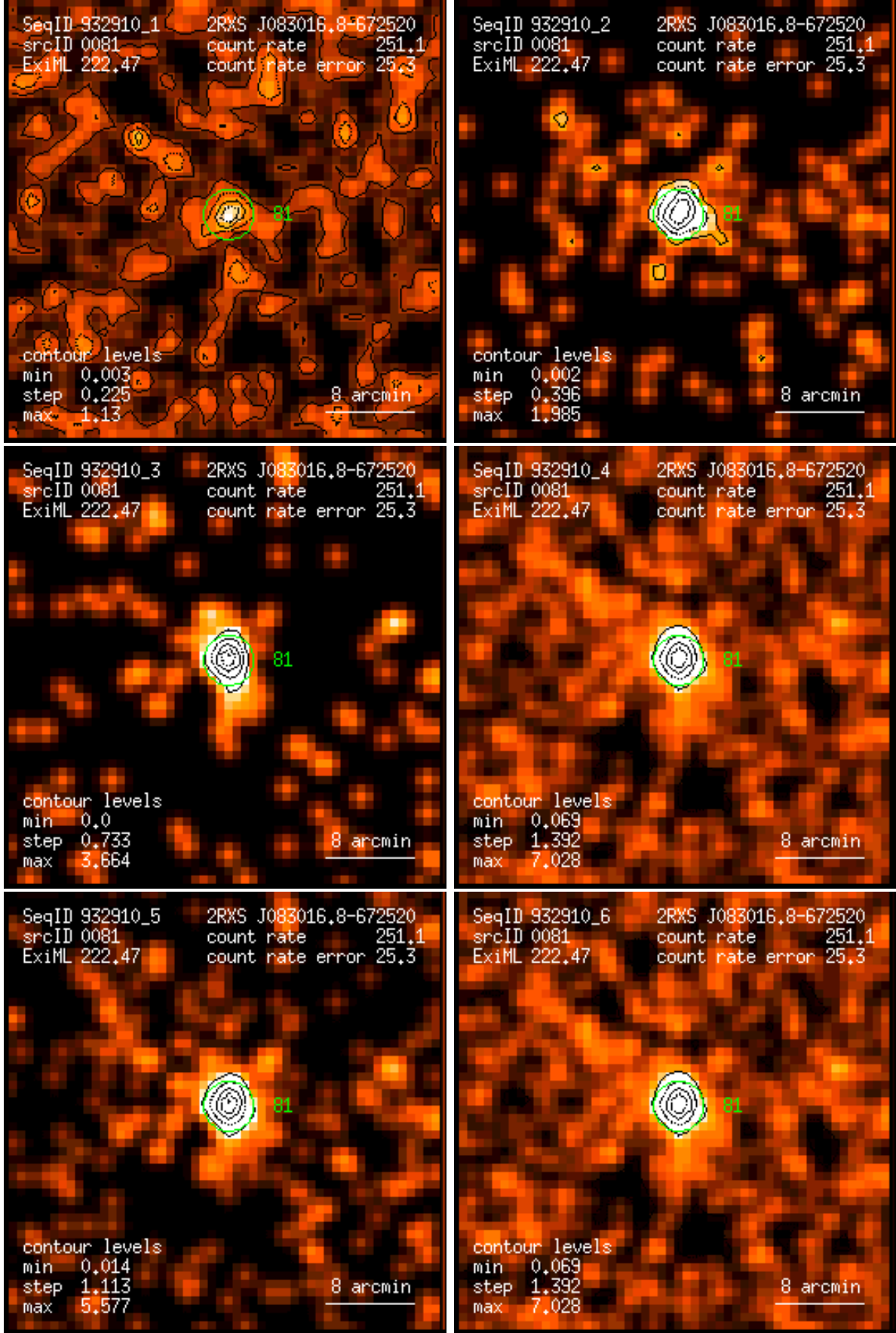
Figure 81: RASS 932910: detection 0081: band rate images, Gaussian filter: (1) PSPC channels 11 – 41, (2) 52 – 90, (3) 91 – 201, (4) 11 – 235, (5) 52 – 201, (6) 11 – 201. Broad band rates in counts/ks. Band rate contour levels in counts/ks/arcmin 2 .
