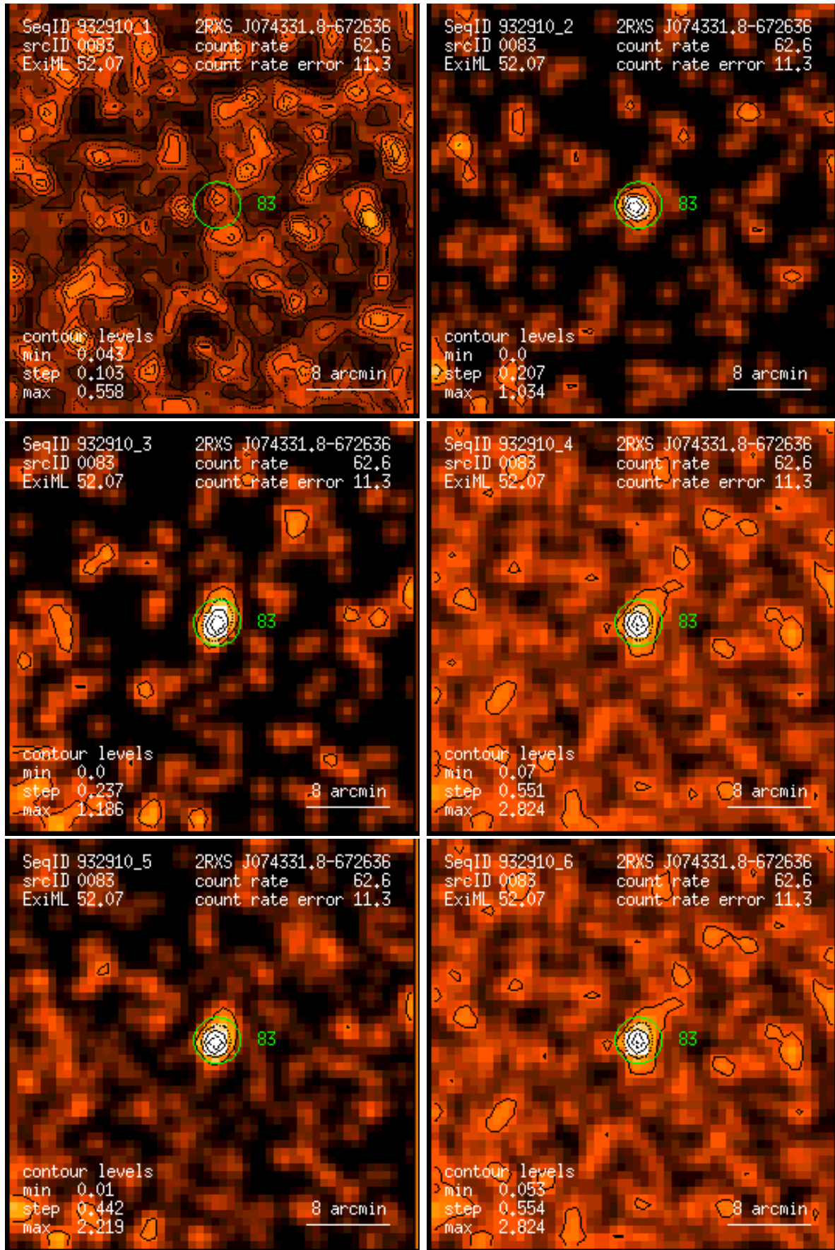
Figure 83: RASS 932910: detection 0083: band rate images, Gaussian filter: (1) PSPC channels 11 – 41, (2) 52 – 90, (3) 91 – 201, (4) 11 – 235, (5) 52 – 201, (6) 11 – 201. Broad band rates in counts/ks. Band rate contour levels in counts/ks/arcmin 2 .
