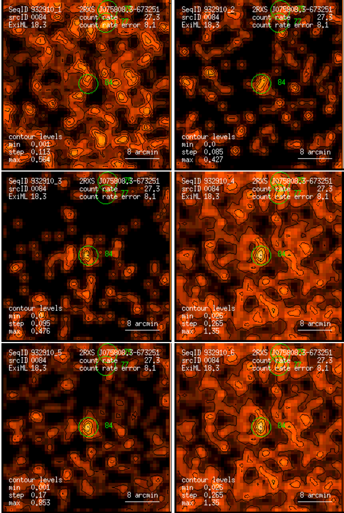
Figure 84: RASS 932910: detection 0084: band rate images, Gaussian filter: (1) PSPC channels 11 – 41, (2) 52 – 90, (3) 91 – 201, (4) 11 – 235, (5) 52 – 201, (6) 11 – 201. Broad band rates in counts/ks. Band rate contour levels in counts/ks/arcmin 2 .
