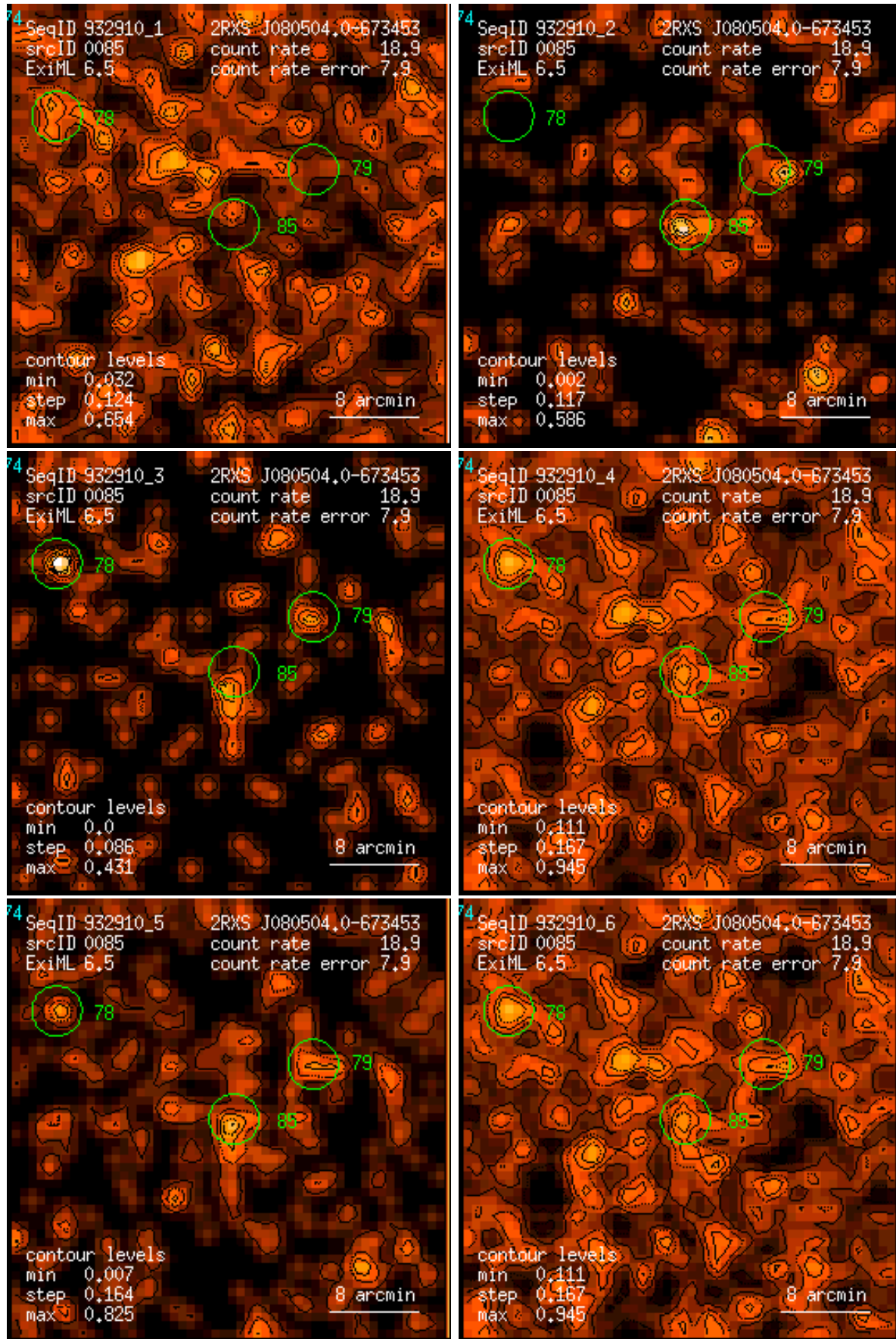
Figure 85: RASS 932910: detection 0085: band rate images, Gaussian filter: (1) PSPC channels 11 – 41, (2) 52 – 90, (3) 91 – 201, (4) 11 – 235, (5) 52 – 201, (6) 11 – 201. Broad band rates in counts/ks. Band rate contour levels in counts/ks/arcmin 2 .
