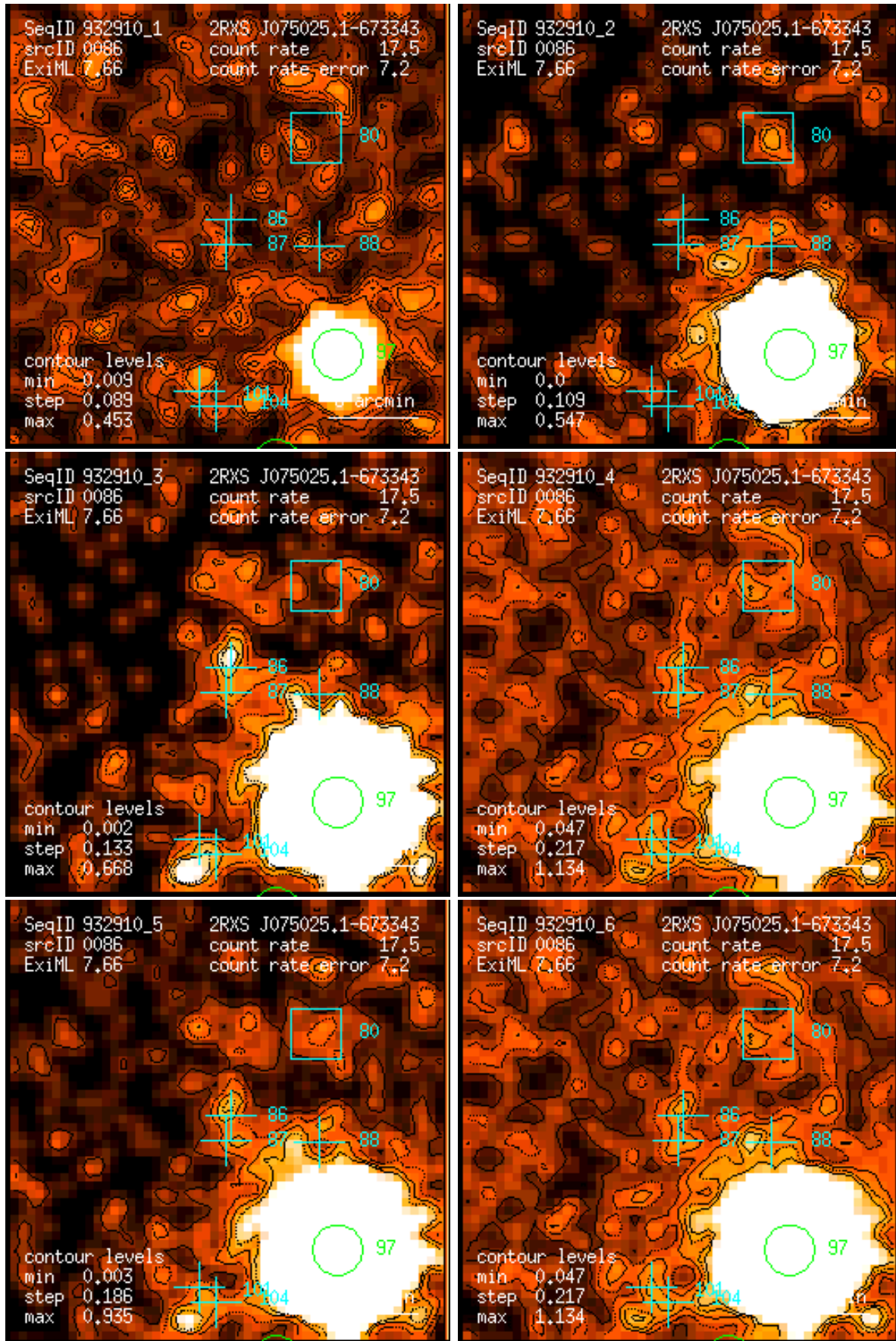
Figure 86: RASS 932910: detection 0086: band rate images, Gaussian filter: (1) PSPC channels 11 – 41, (2) 52 – 90, (3) 91 – 201, (4) 11 – 235, (5) 52 – 201, (6) 11 – 201. Broad band rates in counts/ks. Band rate contour levels in counts/ks/arcmin 2 .
