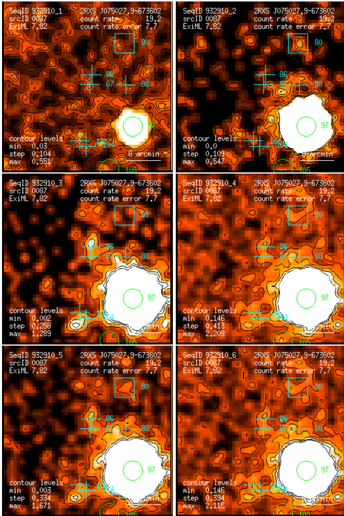
Figure 87: RASS 932910: detection 0087: band rate images, Gaussian filter: (1) PSPC channels 11 – 41, (2) 52 – 90, (3) 91 – 201, (4) 11 – 235, (5) 52 – 201, (6) 11 – 201. Broad band rates in counts/ks. Band rate contour levels in counts/ks/arcmin 2 .
