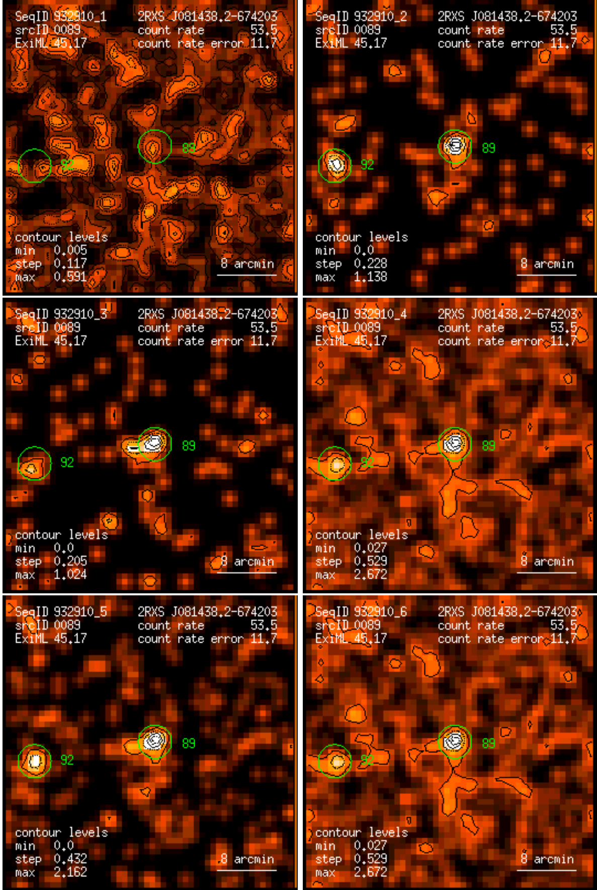
Figure 89: RASS 932910: detection 0089: band rate images, Gaussian filter: (1) PSPC channels 11 – 41, (2) 52 – 90, (3) 91 – 201, (4) 11 – 235, (5) 52 – 201, (6) 11 – 201. Broad band rates in counts/ks. Band rate contour levels in counts/ks/arcmin 2 .
