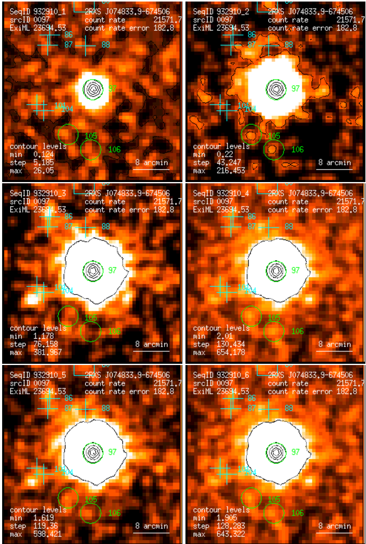
Figure 97: RASS 932910: detection 0097: band rate images, Gaussian filter: (1) PSPC channels 11 – 41, (2) 52 – 90, (3) 91 – 201, (4) 11 – 235, (5) 52 – 201, (6) 11 – 201. Broad band rates in counts/ks. Band rate contour levels in counts/ks/arcmin 2 .
