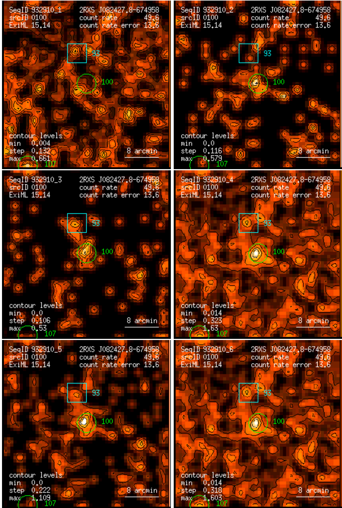
Figure 100: RASS 932910: detection 0100: band rate images, Gaussian filter: (1) PSPC channels 11 – 41, (2) 52 – 90, (3) 91 – 201, (4) 11 – 235, (5) 52 – 201, (6) 11 – 201. Broad band rates in counts/ks. Band rate contour levels in counts/ks/arcmin 2 .
