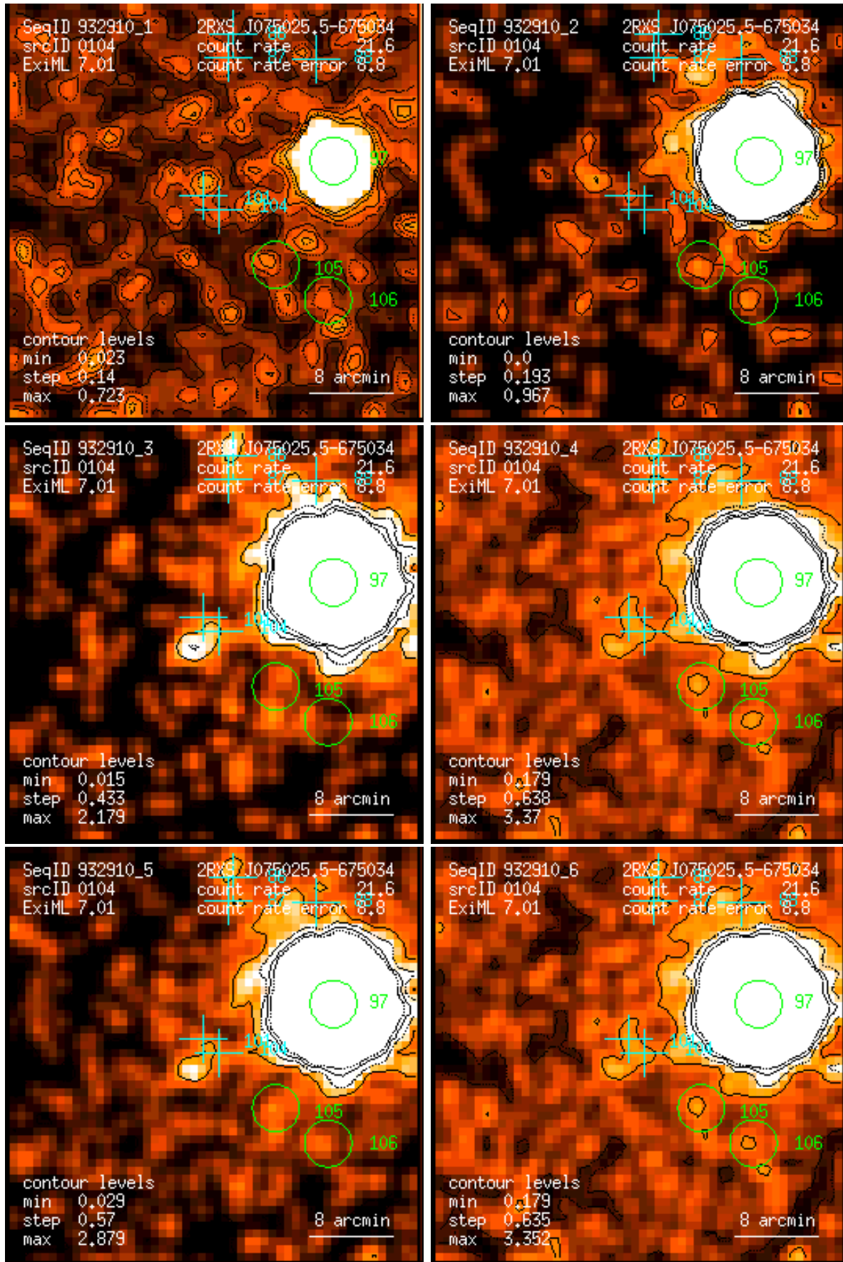
Figure 104: RASS 932910: detection 0104: band rate images, Gaussian filter: (1) PSPC channels 11 – 41, (2) 52 – 90, (3) 91 – 201, (4) 11 – 235, (5) 52 – 201, (6) 11 – 201. Broad band rates in counts/ks. Band rate contour levels in counts/ks/arcmin 2 .
