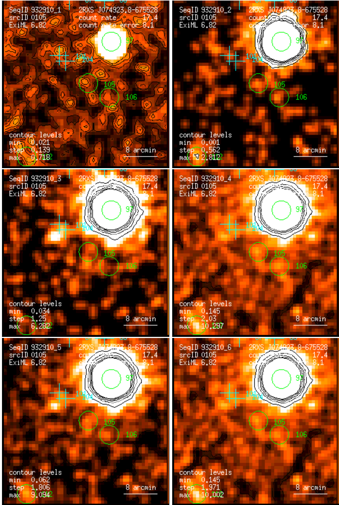
Figure 105: RASS 932910: detection 0105: band rate images, Gaussian filter: (1) PSPC channels 11 – 41, (2) 52 – 90, (3) 91 – 201, (4) 11 – 235, (5) 52 – 201, (6) 11 – 201. Broad band rates in counts/ks. Band rate contour levels in counts/ks/arcmin 2 .
