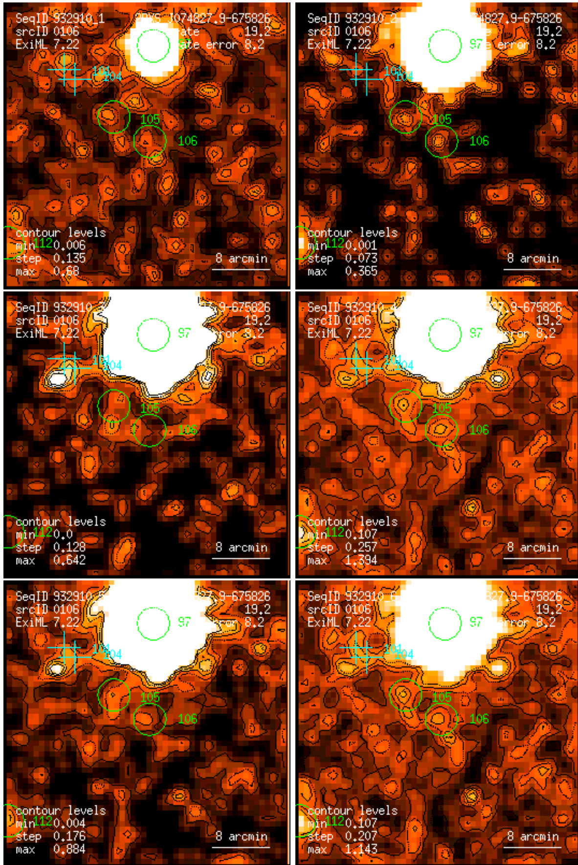
Figure 106: RASS 932910: detection 0106: band rate images, Gaussian filter: (1) PSPC channels 11 – 41, (2) 52 – 90, (3) 91 – 201, (4) 11 – 235, (5) 52 – 201, (6) 11 – 201. Broad band rates in counts/ks. Band rate contour levels in counts/ks/arcmin 2 .
