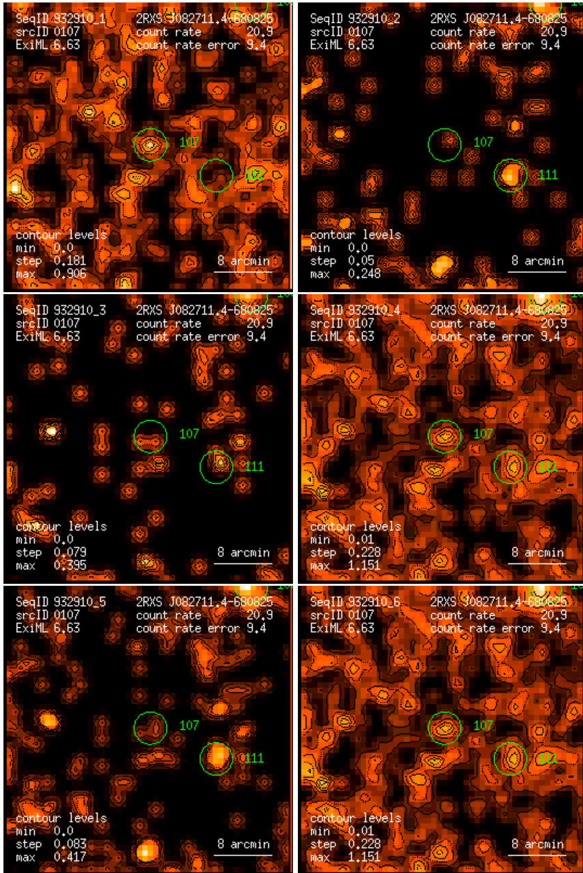
Figure 107: RASS 932910: detection 0107: band rate images, Gaussian filter: (1) PSPC channels 11 – 41, (2) 52 – 90, (3) 91 – 201, (4) 11 – 235, (5) 52 – 201, (6) 11 – 201. Broad band rates in counts/ks. Band rate contour levels in counts/ks/arcmin 2 .
