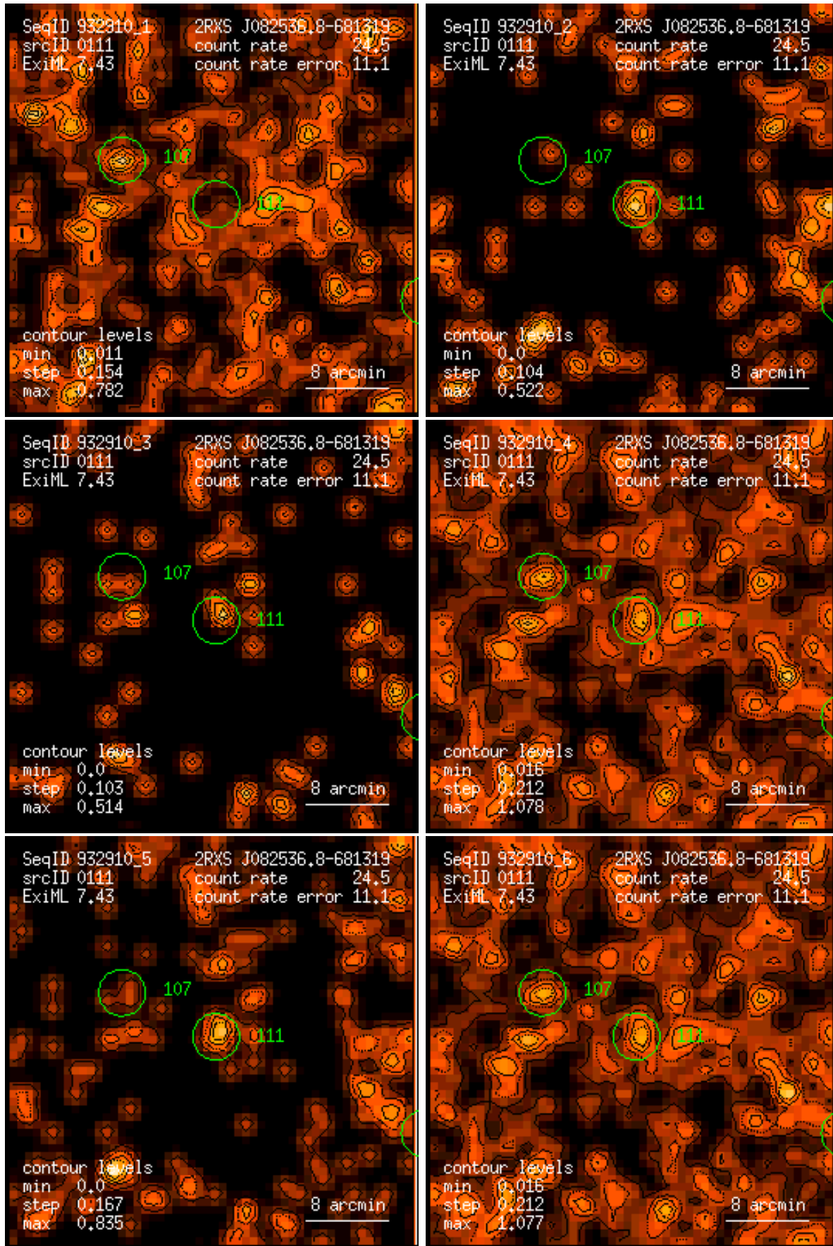
Figure 111: RASS 932910: detection 0111: band rate images, Gaussian filter: (1) PSPC channels 11 – 41, (2) 52 – 90, (3) 91 – 201, (4) 11 – 235, (5) 52 – 201, (6) 11 – 201. Broad band rates in counts/ks. Band rate contour levels in counts/ks/arcmin 2 .
