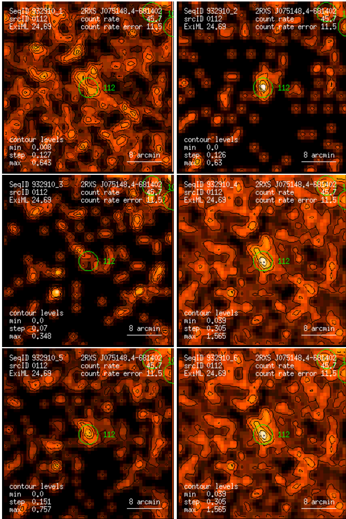
Figure 112: RASS 932910: detection 0112: band rate images, Gaussian filter: (1) PSPC channels 11 – 41, (2) 52 – 90, (3) 91 – 201, (4) 11 – 235, (5) 52 – 201, (6) 11 – 201. Broad band rates in counts/ks. Band rate contour levels in counts/ks/arcmin 2 .
