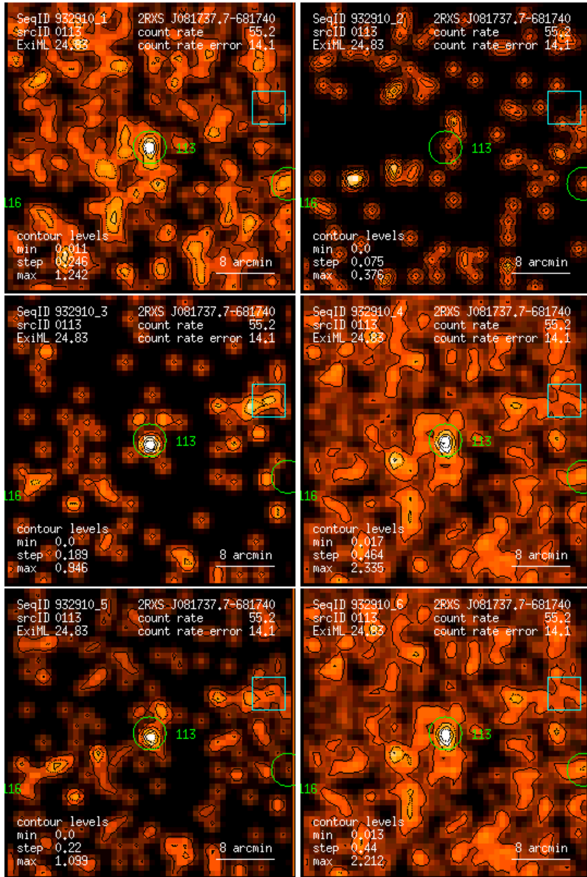
Figure 113: RASS 932910: detection 0113: band rate images, Gaussian filter: (1) PSPC channels 11 – 41, (2) 52 – 90, (3) 91 – 201, (4) 11 – 235, (5) 52 – 201, (6) 11 – 201. Broad band rates in counts/ks. Band rate contour levels in counts/ks/arcmin 2 .
