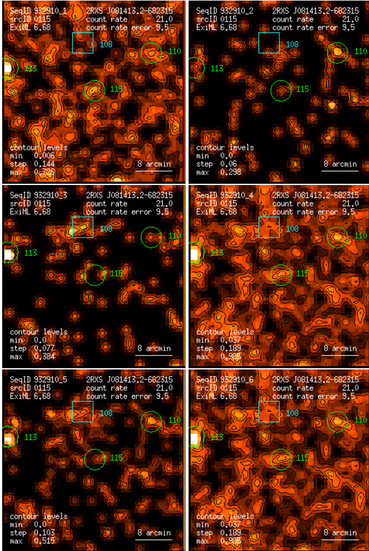
Figure 115: RASS 932910: detection 0115: band rate images, Gaussian filter: (1) PSPC channels 11 – 41, (2) 52 – 90, (3) 91 – 201, (4) 11 – 235, (5) 52 – 201, (6) 11 – 201. Broad band rates in counts/ks. Band rate contour levels in counts/ks/arcmin 2 .
