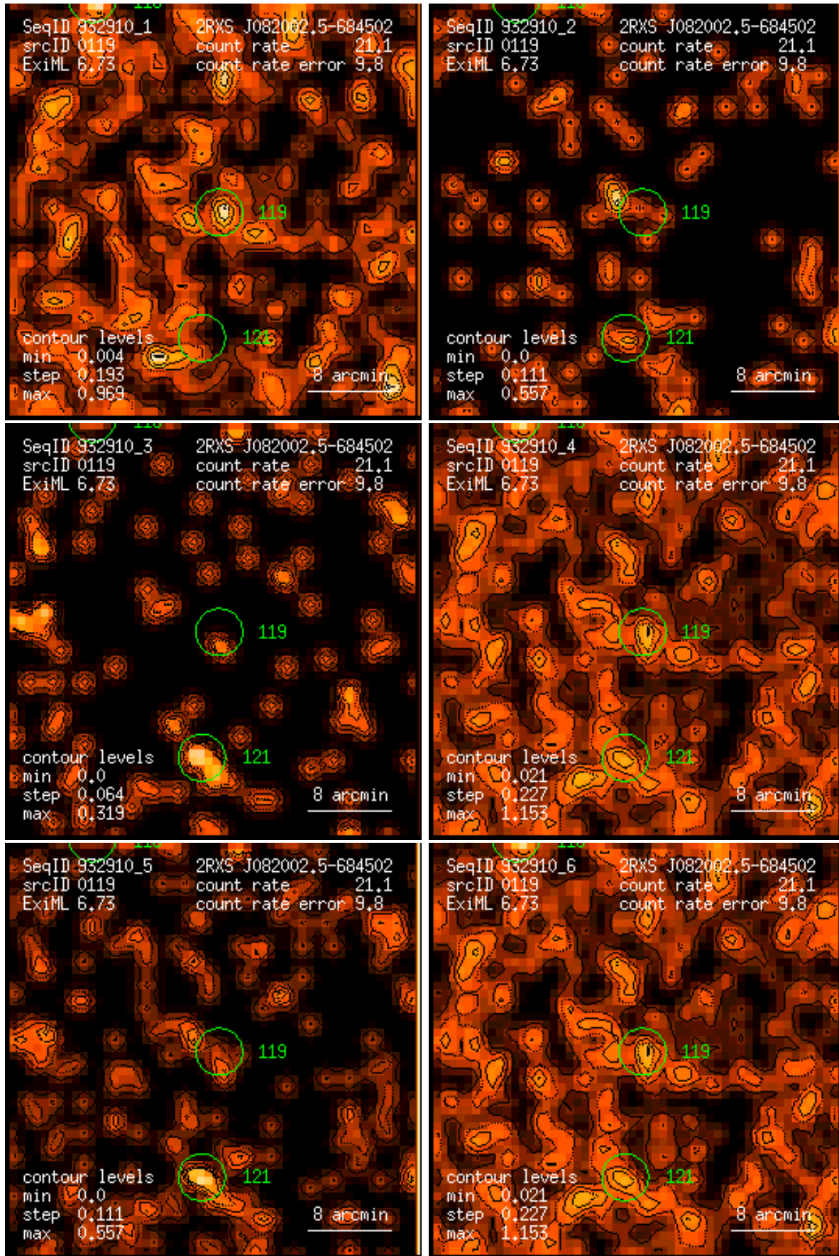
Figure 119: RASS 932910: detection 0119: band rate images, Gaussian filter: (1) PSPC channels 11 – 41, (2) 52 – 90, (3) 91 – 201, (4) 11 – 235, (5) 52 – 201, (6) 11 – 201. Broad band rates in counts/ks. Band rate contour levels in counts/ks/arcmin 2 .
