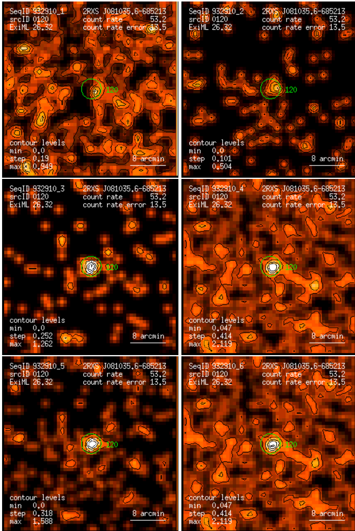
Figure 120: RASS 932910: detection 0120: band rate images, Gaussian filter: (1) PSPC channels 11 – 41, (2) 52 – 90, (3) 91 – 201, (4) 11 – 235, (5) 52 – 201, (6) 11 – 201. Broad band rates in counts/ks. Band rate contour levels in counts/ks/arcmin 2 .
