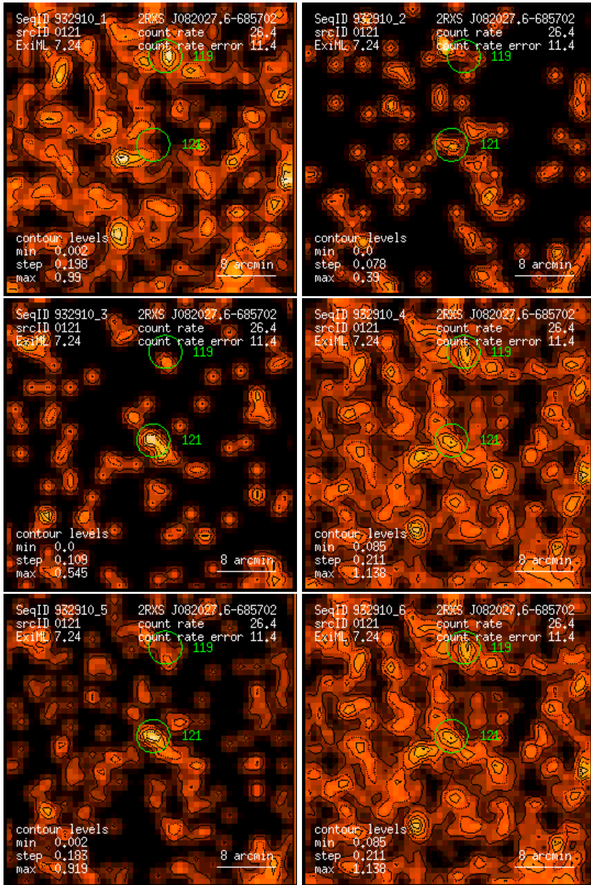
Figure 121: RASS 932910: detection 0121: band rate images, Gaussian filter: (1) PSPC channels 11 – 41, (2) 52 – 90, (3) 91 – 201, (4) 11 – 235, (5) 52 – 201, (6) 11 – 201. Broad band rates in counts/ks. Band rate contour levels in counts/ks/arcmin 2 .
