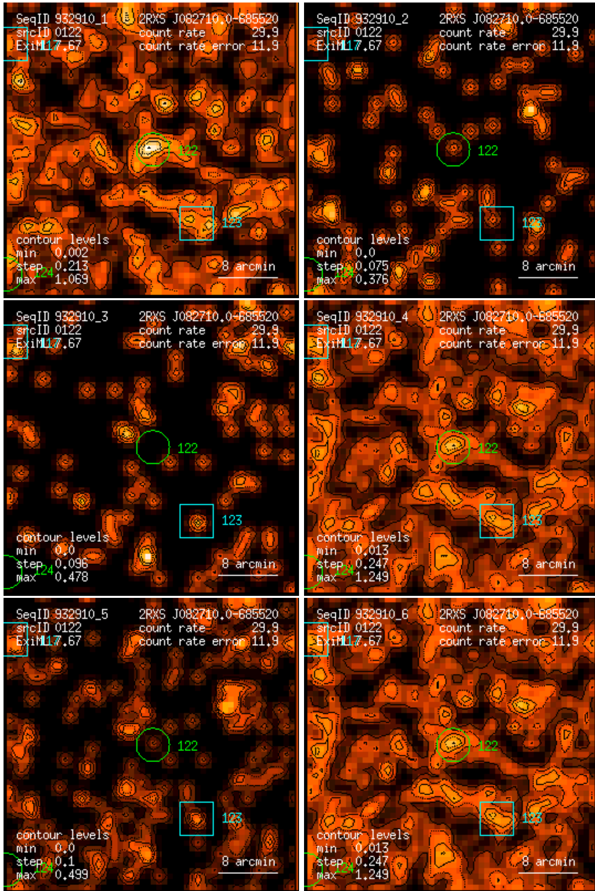
Figure 122: RASS 932910: detection 0122: band rate images, Gaussian filter: (1) PSPC channels 11 – 41, (2) 52 – 90, (3) 91 – 201, (4) 11 – 235, (5) 52 – 201, (6) 11 – 201. Broad band rates in counts/ks. Band rate contour levels in counts/ks/arcmin 2 .
