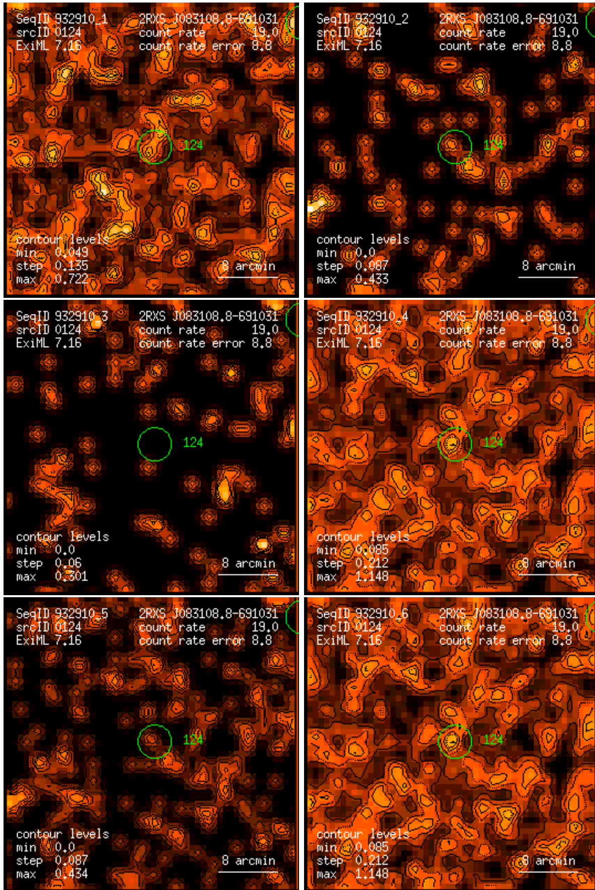
Figure 124: RASS 932910: detection 0124: band rate images, Gaussian filter: (1) PSPC channels 11 – 41, (2) 52 – 90, (3) 91 – 201, (4) 11 – 235, (5) 52 – 201, (6) 11 – 201. Broad band rates in counts/ks. Band rate contour levels in counts/ks/arcmin 2 .
