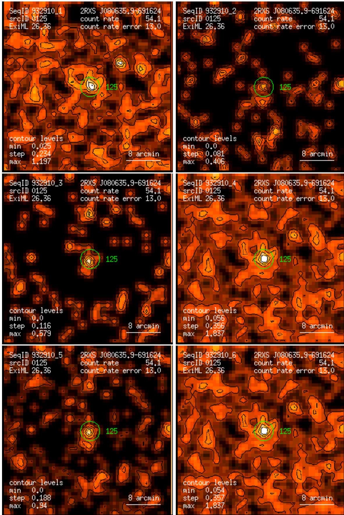
Figure 125: RASS 932910: detection 0125: band rate images, Gaussian filter: (1) PSPC channels 11 – 41, (2) 52 – 90, (3) 91 – 201, (4) 11 – 235, (5) 52 – 201, (6) 11 – 201. Broad band rates in counts/ks. Band rate contour levels in counts/ks/arcmin 2 .
