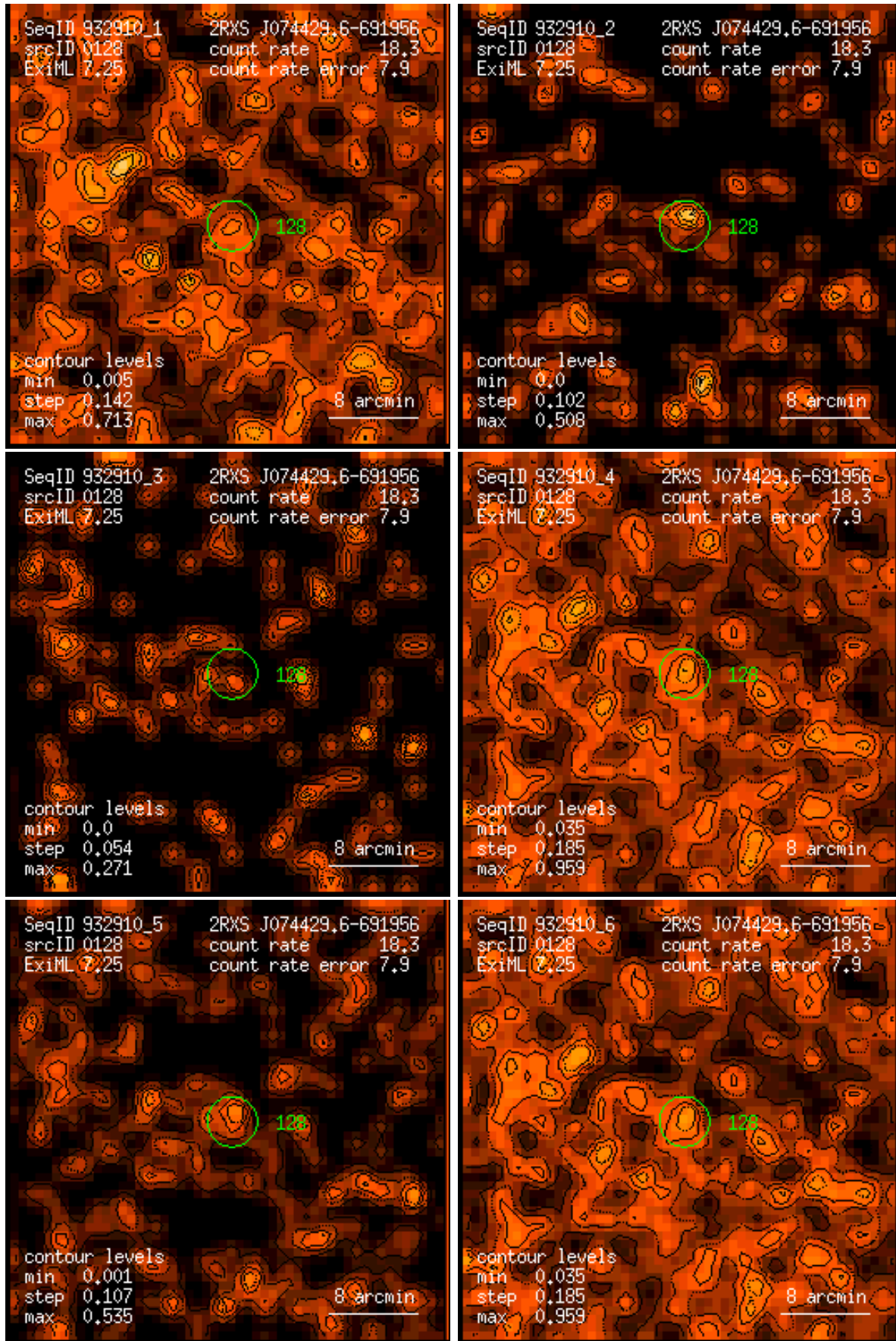
Figure 128: RASS 932910: detection 0128: band rate images, Gaussian filter: (1) PSPC channels 11 – 41, (2) 52 – 90, (3) 91 – 201, (4) 11 – 235, (5) 52 – 201, (6) 11 – 201. Broad band rates in counts/ks. Band rate contour levels in counts/ks/arcmin 2 .
