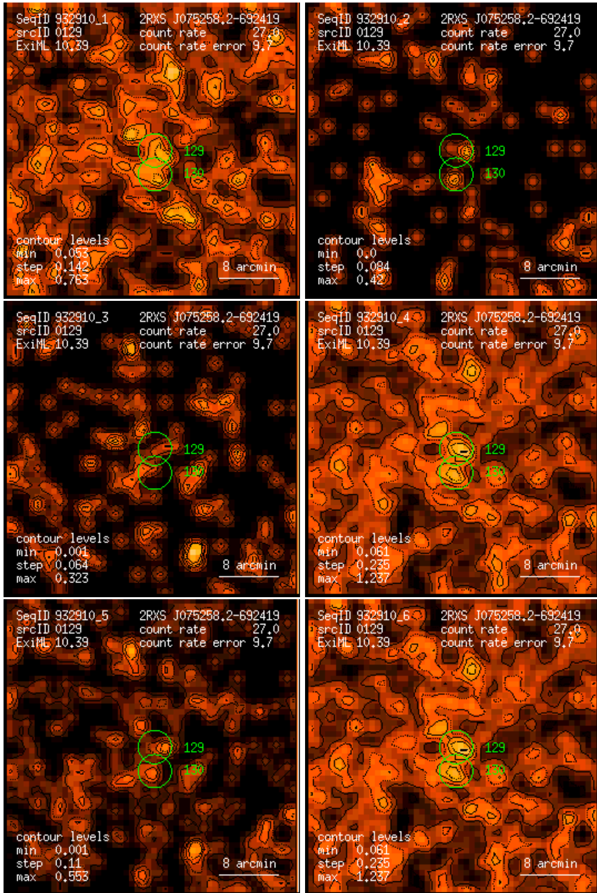
Figure 129: RASS 932910: detection 0129: band rate images, Gaussian filter: (1) PSPC channels 11 – 41, (2) 52 – 90, (3) 91 – 201, (4) 11 – 235, (5) 52 – 201, (6) 11 – 201. Broad band rates in counts/ks. Band rate contour levels in counts/ks/arcmin 2 .
