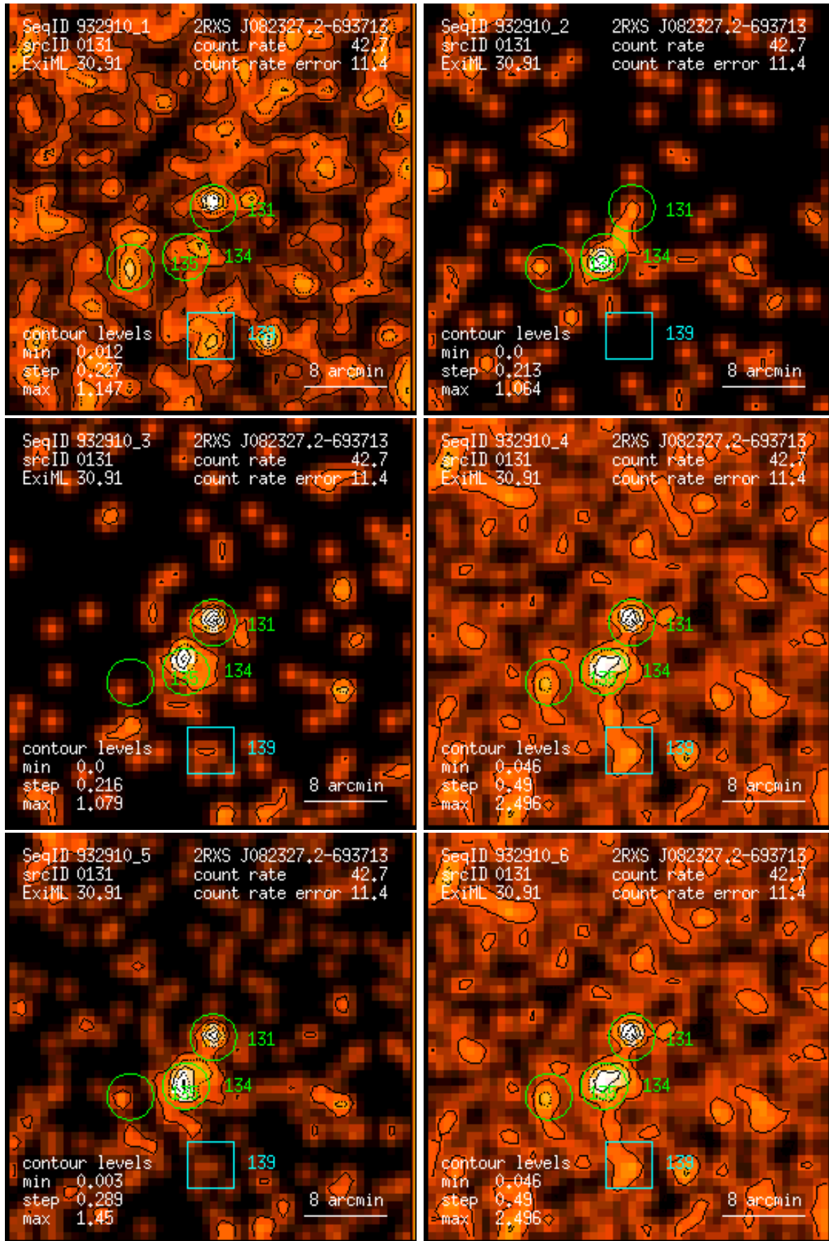
Figure 131: RASS 932910: detection 0131: band rate images, Gaussian filter: (1) PSPC channels 11 – 41, (2) 52 – 90, (3) 91 – 201, (4) 11 – 235, (5) 52 – 201, (6) 11 – 201. Broad band rates in counts/ks. Band rate contour levels in counts/ks/arcmin 2 .
