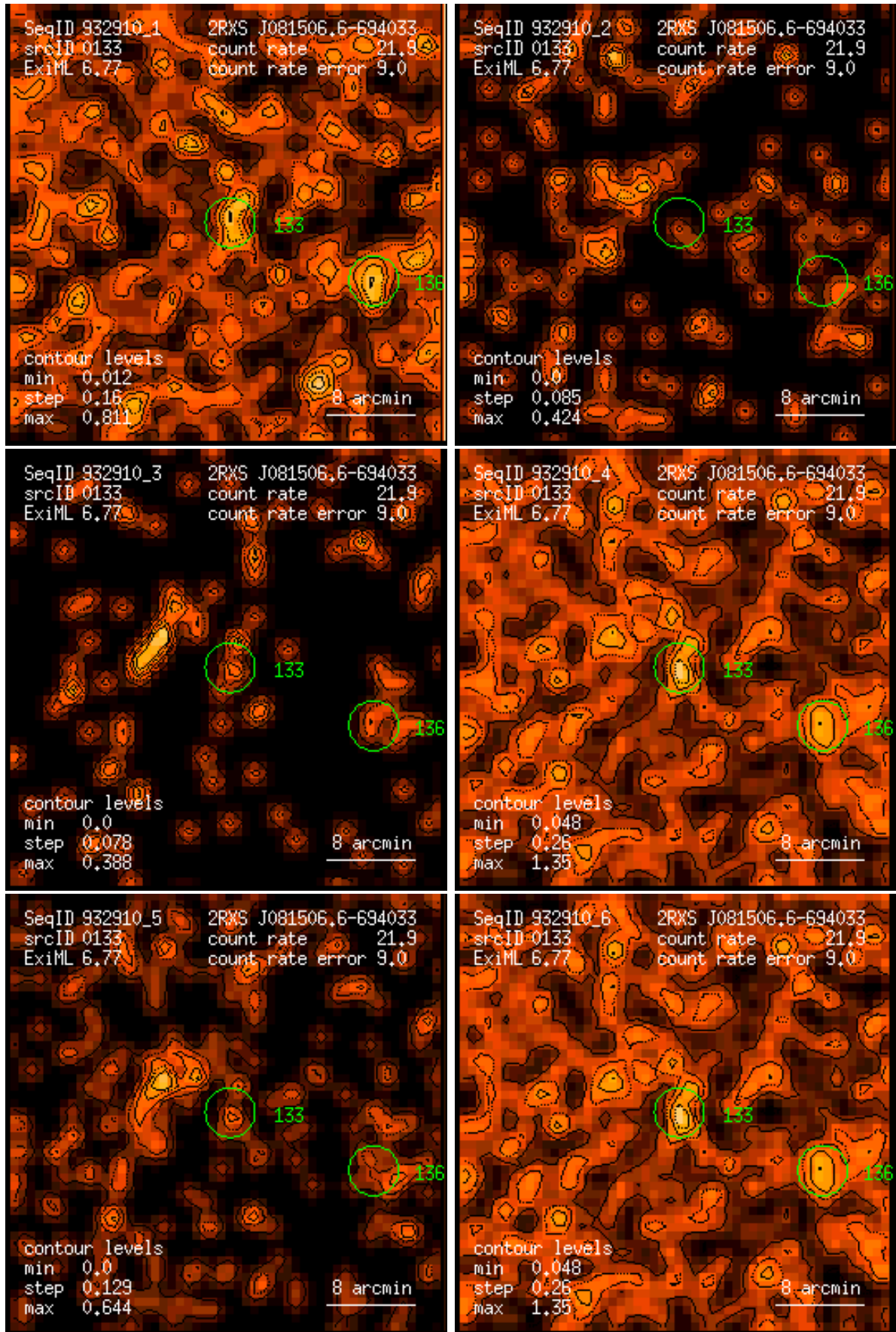
Figure 133: RASS 932910: detection 0133: band rate images, Gaussian filter: (1) PSPC channels 11 – 41, (2) 52 – 90, (3) 91 – 201, (4) 11 – 235, (5) 52 – 201, (6) 11 – 201. Broad band rates in counts/ks. Band rate contour levels in counts/ks/arcmin 2 .
