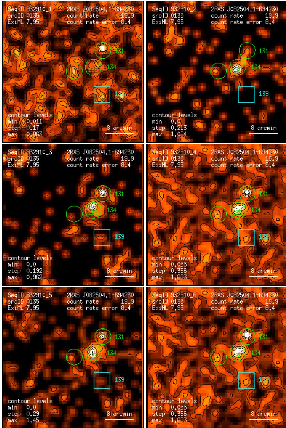
Figure 135: RASS 932910: detection 0135: band rate images, Gaussian filter: (1) PSPC channels 11 – 41, (2) 52 – 90, (3) 91 – 201, (4) 11 – 235, (5) 52 – 201, (6) 11 – 201. Broad band rates in counts/ks. Band rate contour levels in counts/ks/arcmin 2 .
