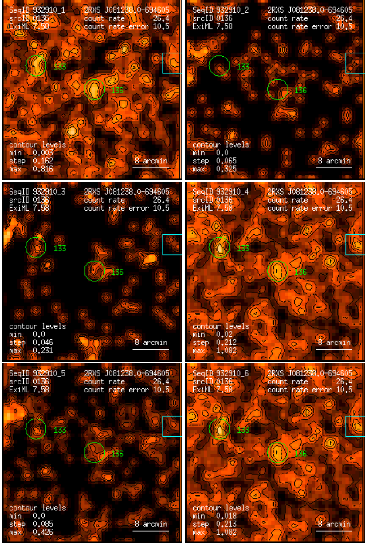
Figure 136: RASS 932910: detection 0136: band rate images, Gaussian filter: (1) PSPC channels 11 – 41, (2) 52 – 90, (3) 91 – 201, (4) 11 – 235, (5) 52 – 201, (6) 11 – 201. Broad band rates in counts/ks. Band rate contour levels in counts/ks/arcmin 2 .
