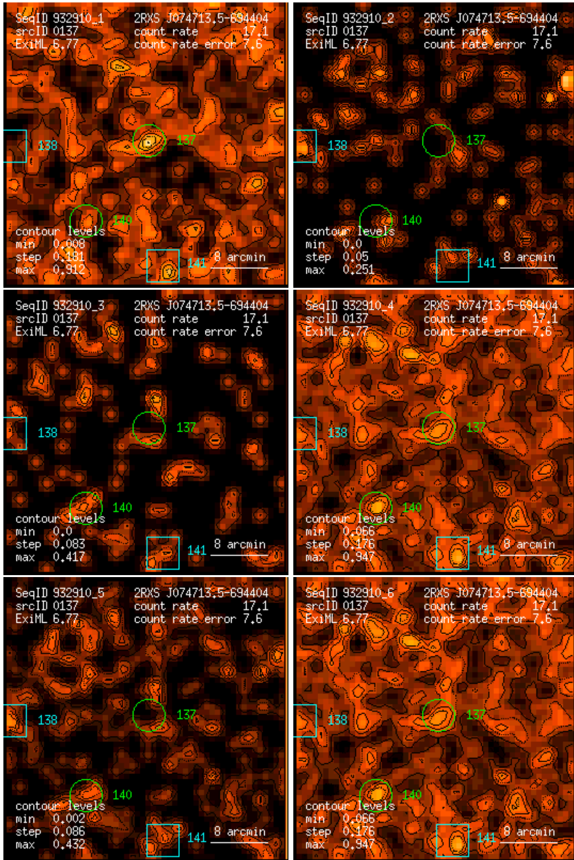
Figure 137: RASS 932910: detection 0137: band rate images, Gaussian filter: (1) PSPC channels 11 – 41, (2) 52 – 90, (3) 91 – 201, (4) 11 – 235, (5) 52 – 201, (6) 11 – 201. Broad band rates in counts/ks. Band rate contour levels in counts/ks/arcmin 2 .
