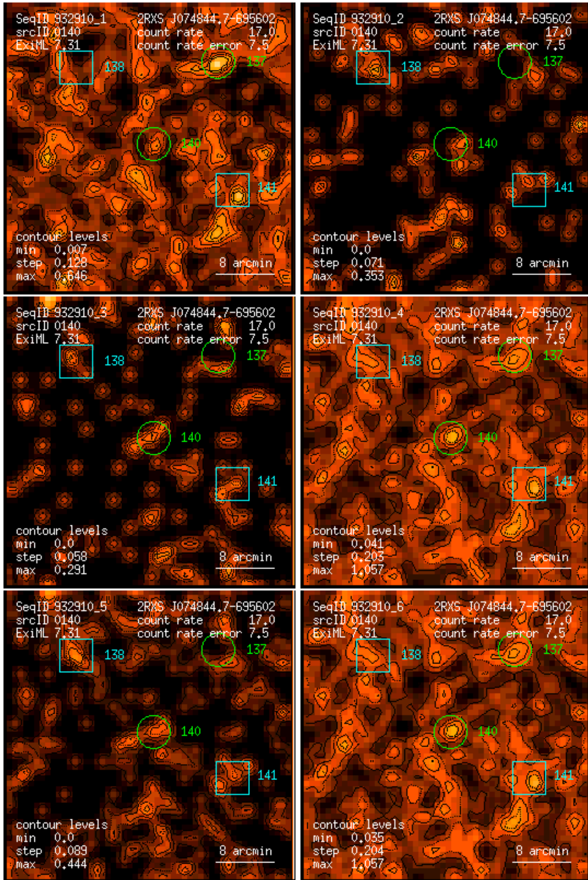
Figure 140: RASS 932910: detection 0140: band rate images, Gaussian filter: (1) PSPC channels 11 – 41, (2) 52 – 90, (3) 91 – 201, (4) 11 – 235, (5) 52 – 201, (6) 11 – 201. Broad band rates in counts/ks. Band rate contour levels in counts/ks/arcmin 2 .
