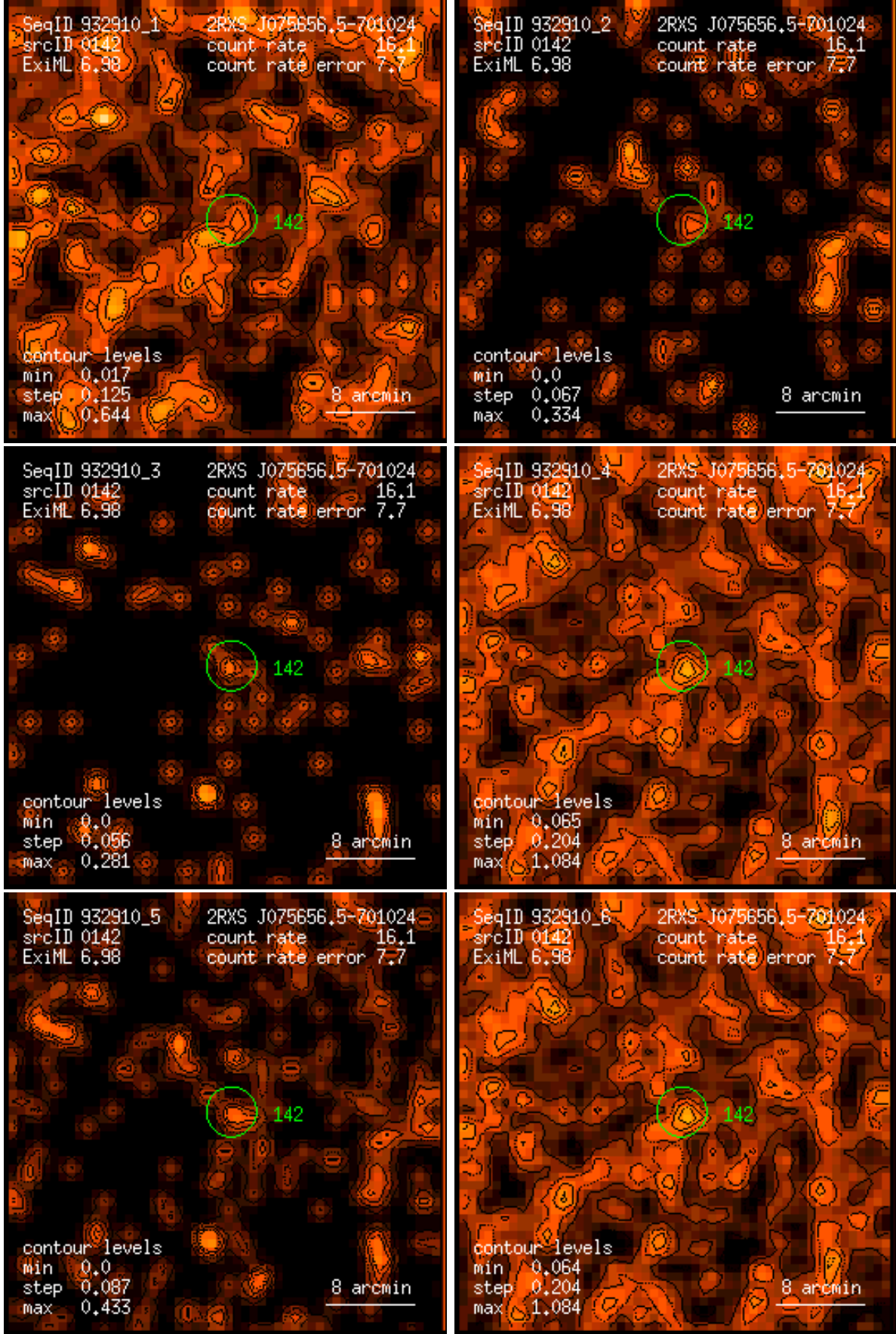
Figure 142: RASS 932910: detection 0142: band rate images, Gaussian filter: (1) PSPC channels 11 – 41, (2) 52 – 90, (3) 91 – 201, (4) 11 – 235, (5) 52 – 201, (6) 11 – 201. Broad band rates in counts/ks. Band rate contour levels in counts/ks/arcmin 2 .
