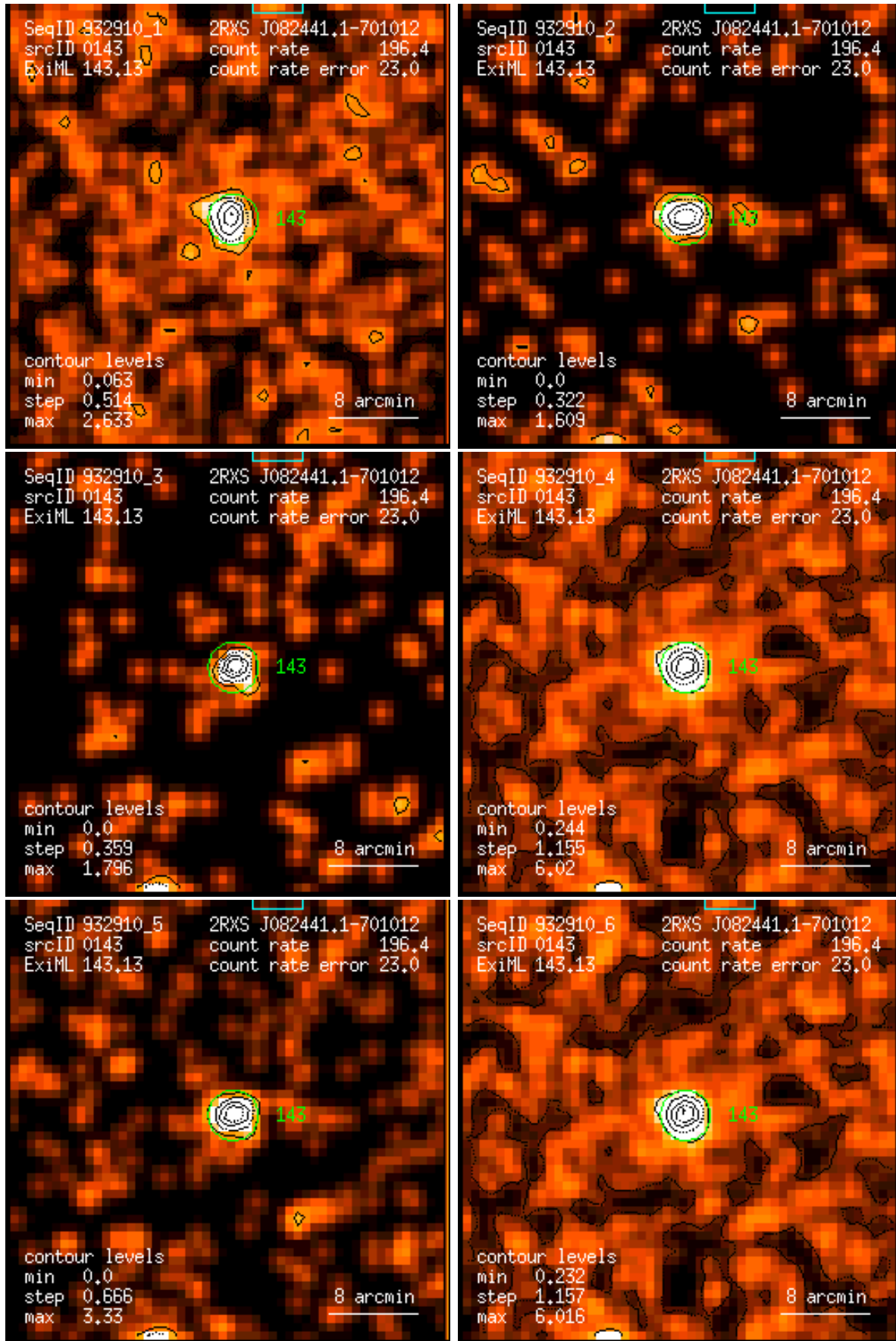
Figure 143: RASS 932910: detection 0143: band rate images, Gaussian filter: (1) PSPC channels 11 – 41, (2) 52 – 90, (3) 91 – 201, (4) 11 – 235, (5) 52 – 201, (6) 11 – 201. Broad band rates in counts/ks. Band rate contour levels in counts/ks/arcmin 2 .
