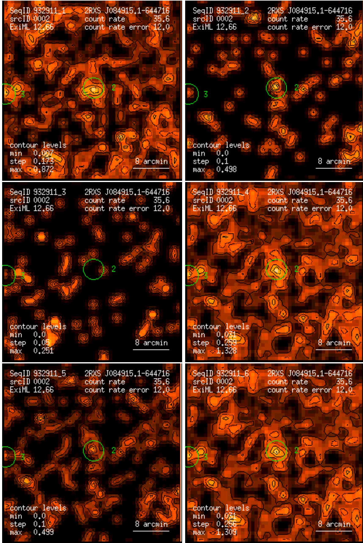
Figure 2: RASS 932911: detection 0002: band rate images, Gaussian filter: (1) PSPC channels 11 – 41, (2) 52 – 90, (3) 91 – 201, (4) 11 – 235, (5) 52 – 201, (6) 11 – 201. Broad band rates in counts/ks. Band rate contour levels in counts/ks/arcmin 2 .
