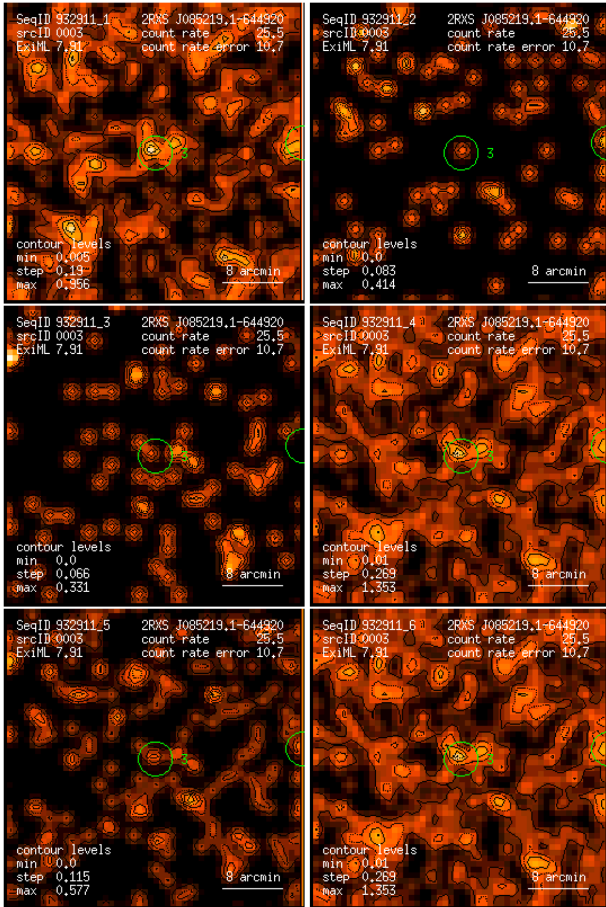
Figure 3: RASS 932911: detection 0003: band rate images, Gaussian filter: (1) PSPC channels 11 – 41, (2) 52 – 90, (3) 91 – 201, (4) 11 – 235, (5) 52 – 201, (6) 11 – 201. Broad band rates in counts/ks. Band rate contour levels in counts/ks/arcmin 2 .
