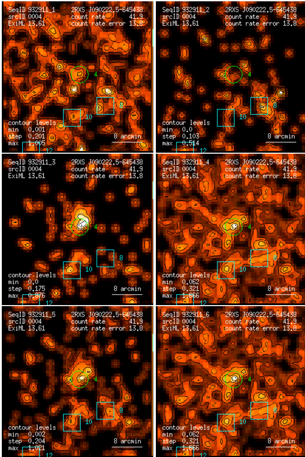
Figure 4: RASS 932911: detection 0004: band rate images, Gaussian filter: (1) PSPC channels 11 – 41, (2) 52 – 90, (3) 91 – 201, (4) 11 – 235, (5) 52 – 201, (6) 11 – 201. Broad band rates in counts/ks. Band rate contour levels in counts/ks/arcmin 2 .
