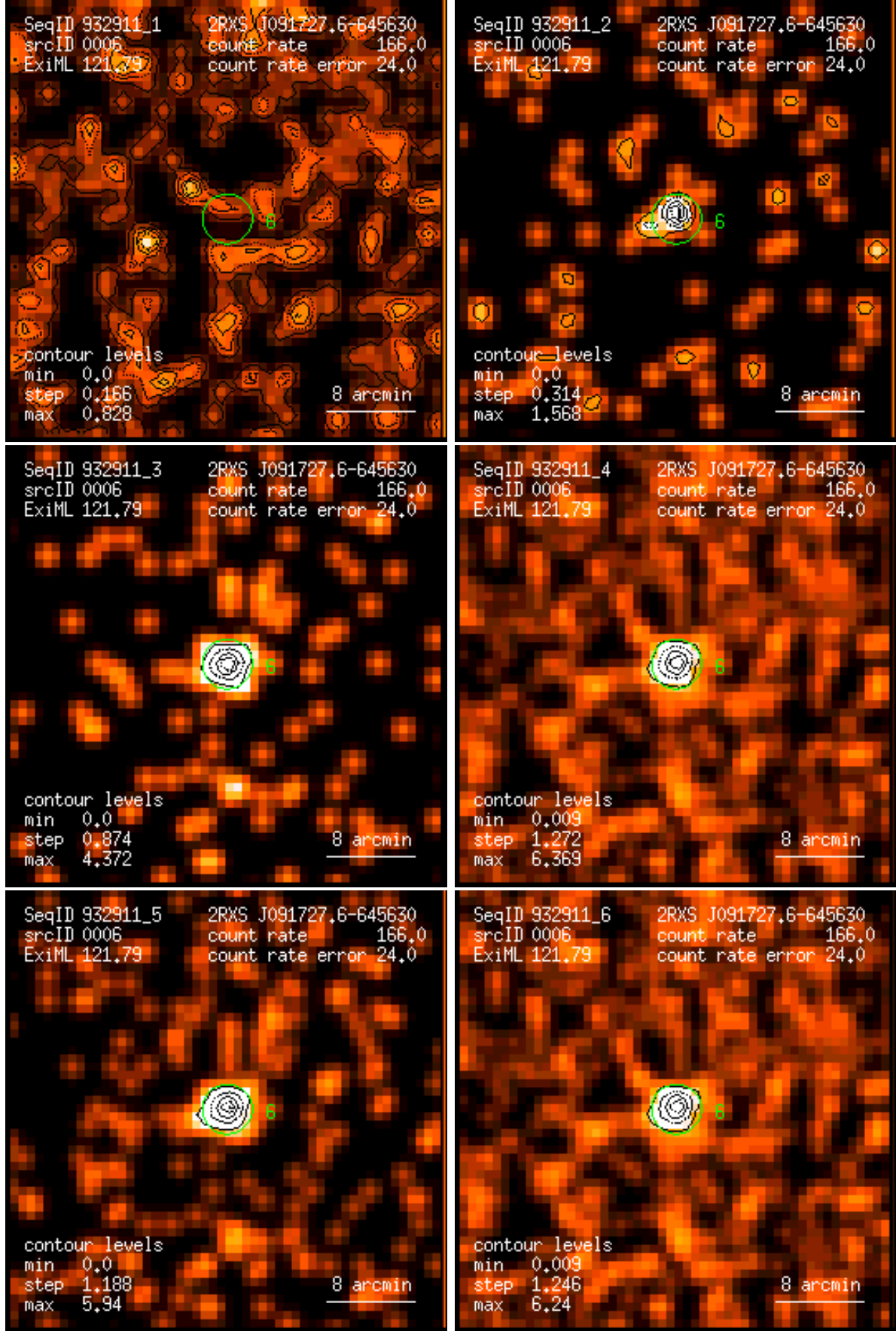
Figure 6: RASS 932911: detection 0006: band rate images, Gaussian filter: (1) PSPC channels 11 – 41, (2) 52 – 90, (3) 91 – 201, (4) 11 – 235, (5) 52 – 201, (6) 11 – 201. Broad band rates in counts/ks. Band rate contour levels in counts/ks/arcmin 2 .
