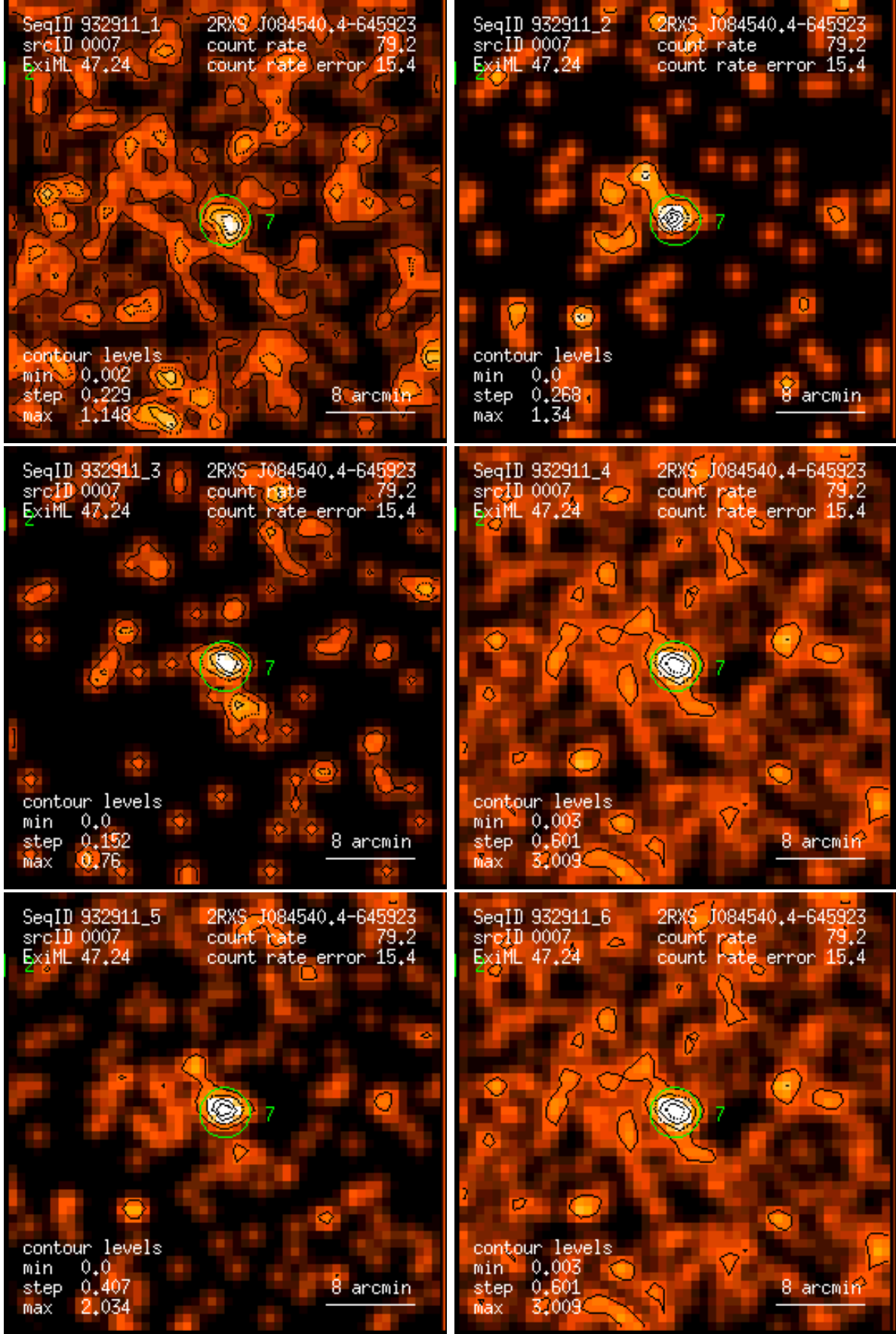
Figure 7: RASS 932911: detection 0007: band rate images, Gaussian filter: (1) PSPC channels 11 – 41, (2) 52 – 90, (3) 91 – 201, (4) 11 – 235, (5) 52 – 201, (6) 11 – 201. Broad band rates in counts/ks. Band rate contour levels in counts/ks/arcmin 2 .
