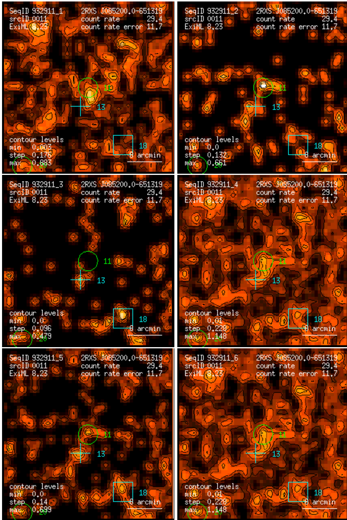
Figure 11: RASS 932911: detection 0011: band rate images, Gaussian filter: (1) PSPC channels 11 – 41, (2) 52 – 90, (3) 91 – 201, (4) 11 – 235, (5) 52 – 201, (6) 11 – 201. Broad band rates in counts/ks. Band rate contour levels in counts/ks/arcmin 2 .
