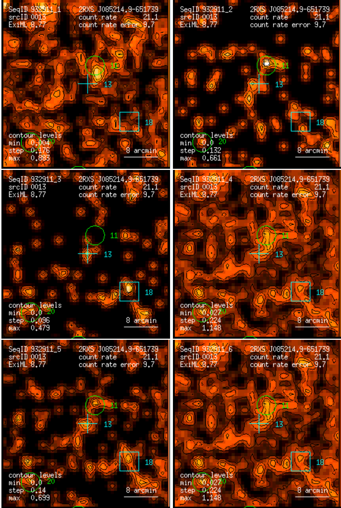
Figure 13: RASS 932911: detection 0013: band rate images, Gaussian filter: (1) PSPC channels 11 – 41, (2) 52 – 90, (3) 91 – 201, (4) 11 – 235, (5) 52 – 201, (6) 11 – 201. Broad band rates in counts/ks. Band rate contour levels in counts/ks/arcmin 2 .
