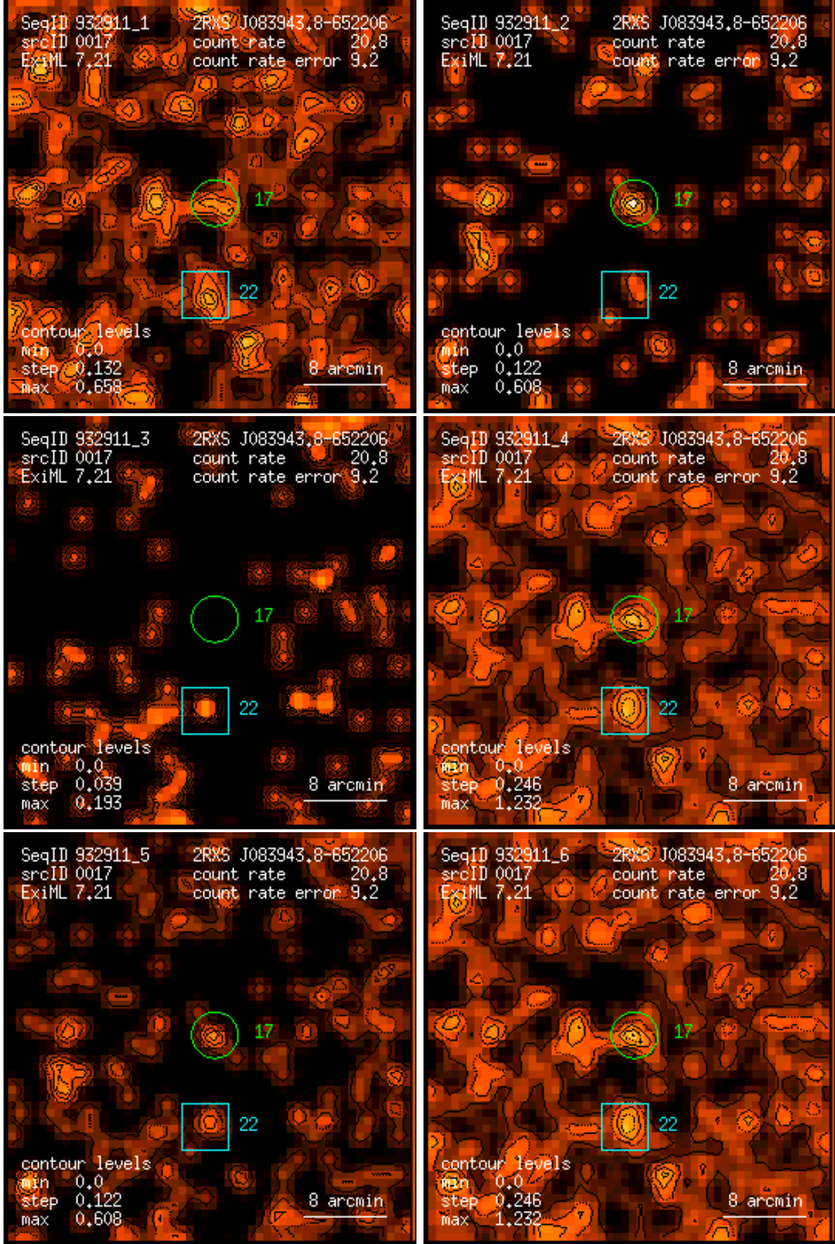
Figure 17: RASS 932911: detection 0017: band rate images, Gaussian filter: (1) PSPC channels 11 – 41, (2) 52 – 90, (3) 91 – 201, (4) 11 – 235, (5) 52 – 201, (6) 11 – 201. Broad band rates in counts/ks. Band rate contour levels in counts/ks/arcmin 2 .
