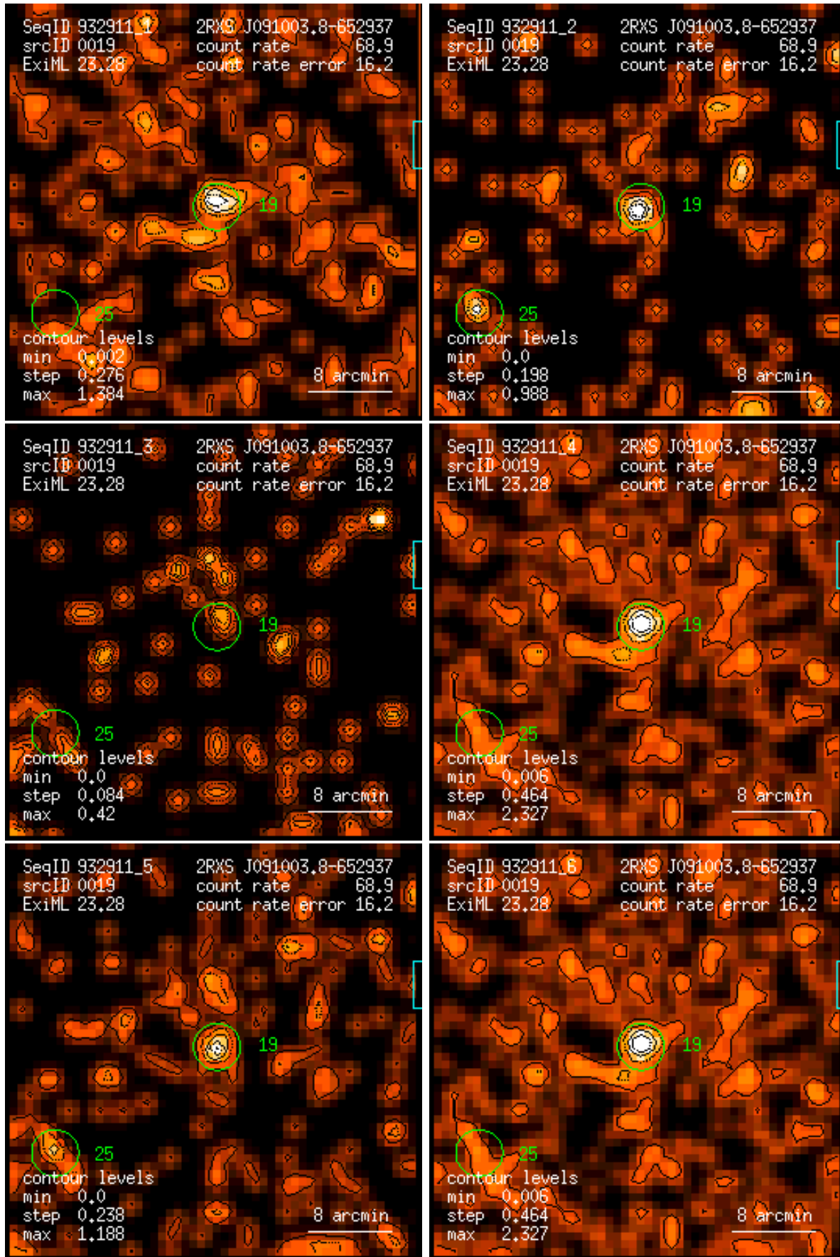
Figure 19: RASS 932911: detection 0019: band rate images, Gaussian filter: (1) PSPC channels 11 – 41, (2) 52 – 90, (3) 91 – 201, (4) 11 – 235, (5) 52 – 201, (6) 11 – 201. Broad band rates in counts/ks. Band rate contour levels in counts/ks/arcmin 2 .
