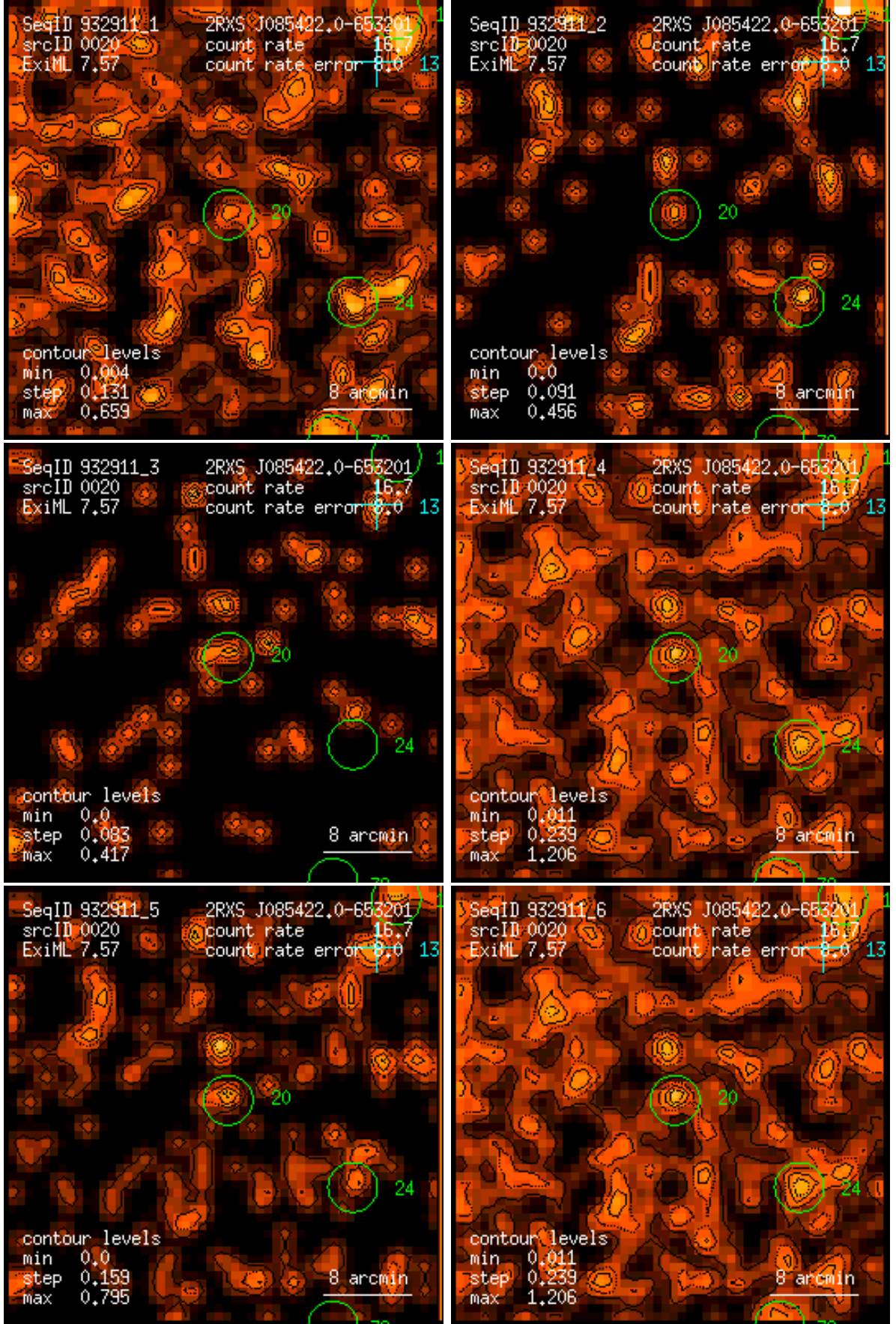
Figure 20: RASS 932911: detection 0020: band rate images, Gaussian filter: (1) PSPC channels 11 – 41, (2) 52 – 90, (3) 91 – 201, (4) 11 – 235, (5) 52 – 201, (6) 11 – 201. Broad band rates in counts/ks. Band rate contour levels in counts/ks/arcmin 2 .
