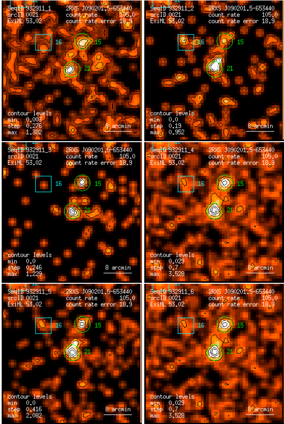
Figure 21: RASS 932911: detection 0021: band rate images, Gaussian filter: (1) PSPC channels 11 – 41, (2) 52 – 90, (3) 91 – 201, (4) 11 – 235, (5) 52 – 201, (6) 11 – 201. Broad band rates in counts/ks. Band rate contour levels in counts/ks/arcmin 2 .
